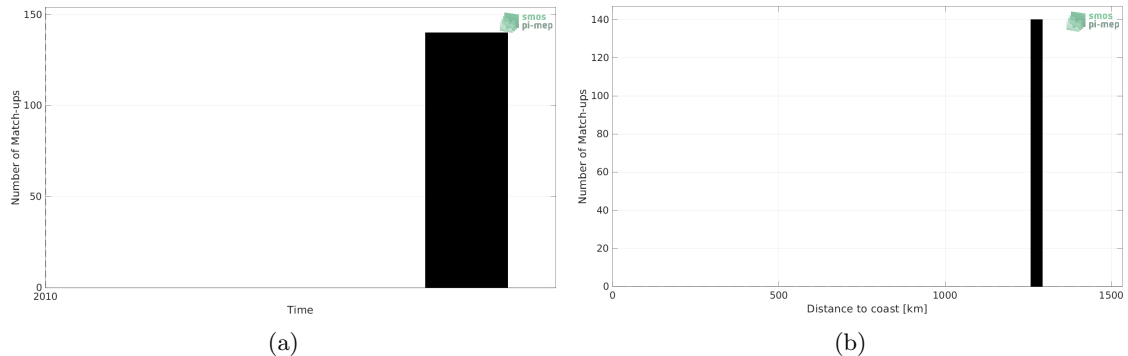
Figure 1: Number of match-ups between TSG (SAMOS) and SMOS SSS L2Q v330 - 0.25 Deg (CATDS-CPDC) SSS as a function of time (a) and as function of the distance to coast (b) over the Congo river plume Pi-MEP region and for the full satellite product period.
