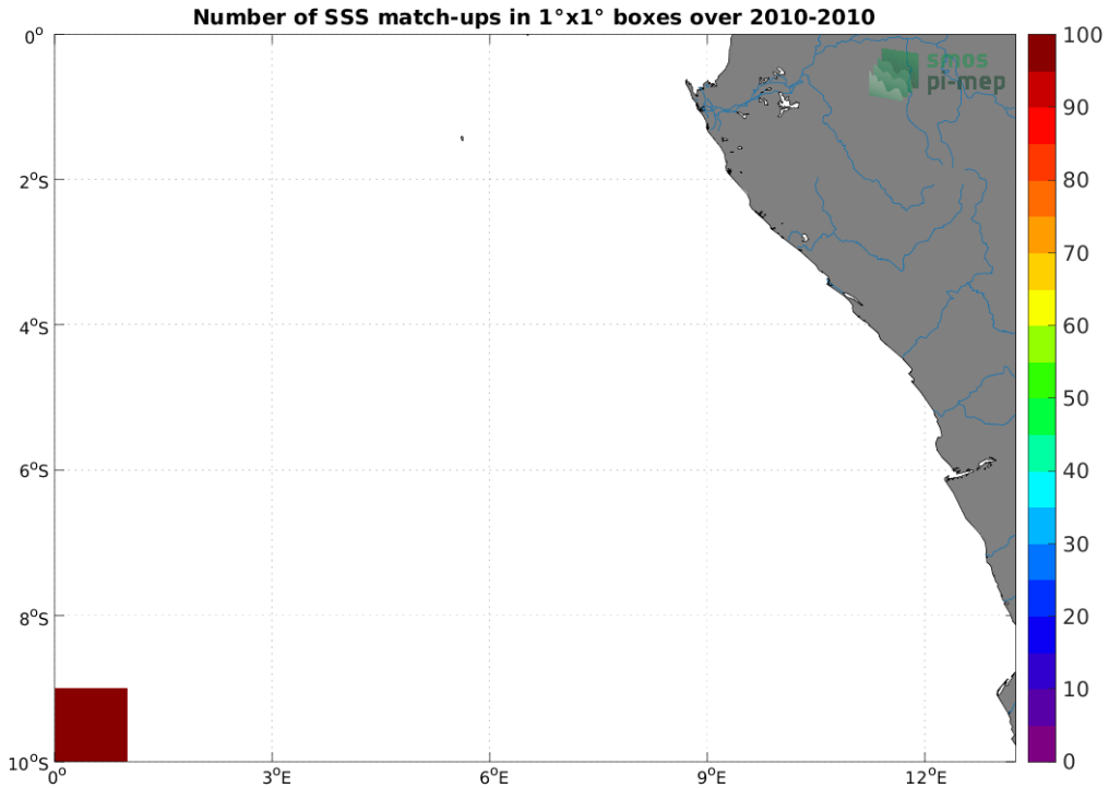
Figure 4: Number of SSS match-ups between TSG (SAMOS) SSS and the SMOS SSS L2Q v330 - 0.25 Deg (CATDS-CPDC) SSS product for the Congo river plume Pi-MEP region over 1^\circ \times 1^\circ boxes and for the full satellite product period.
