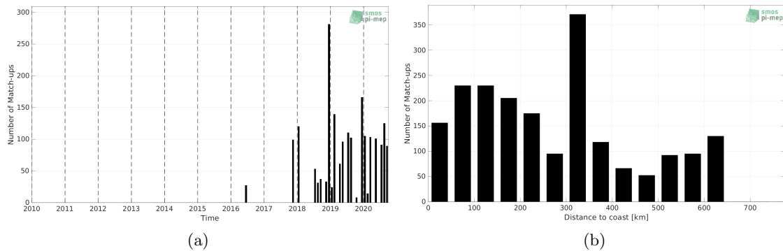
Figure 1: Number of match-ups between TSG (LEGOS-DM) and SMOS SSS L2Q v330 - 0.25 Deg (CATDS-CPDC) SSS as a function of time (a) and as function of the distance to coast (b) over the Congo river plume Pi-MEP region and for the full satellite product period.
