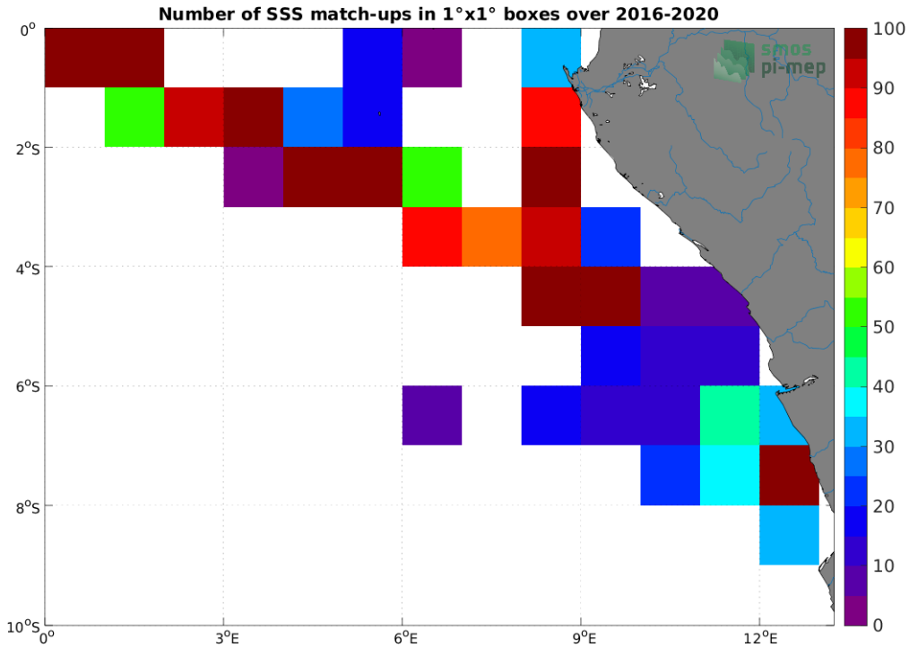
Figure 4: Number of SSS match-ups between TSG (LEGOS-DM) SSS and the SMOS SSS L2Q v330 - 0.25 Deg (CATDS-CPDC) SSS product for the Congo river plume Pi-MEP region over 1^\circ \times 1^\circ boxes and for the full satellite product period.
