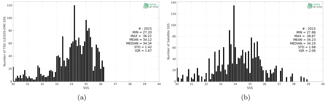
Figure 2: Histograms of SSS from TSG (LEGOS-DM) (a) and SMOS SSS L2Q v330 - 0.25 Deg (CATDS-CPDC) (b) considering all match-up pairs per bins of 0.1 over the Congo river plume Pi-MEP region and for the full satellite product period.
