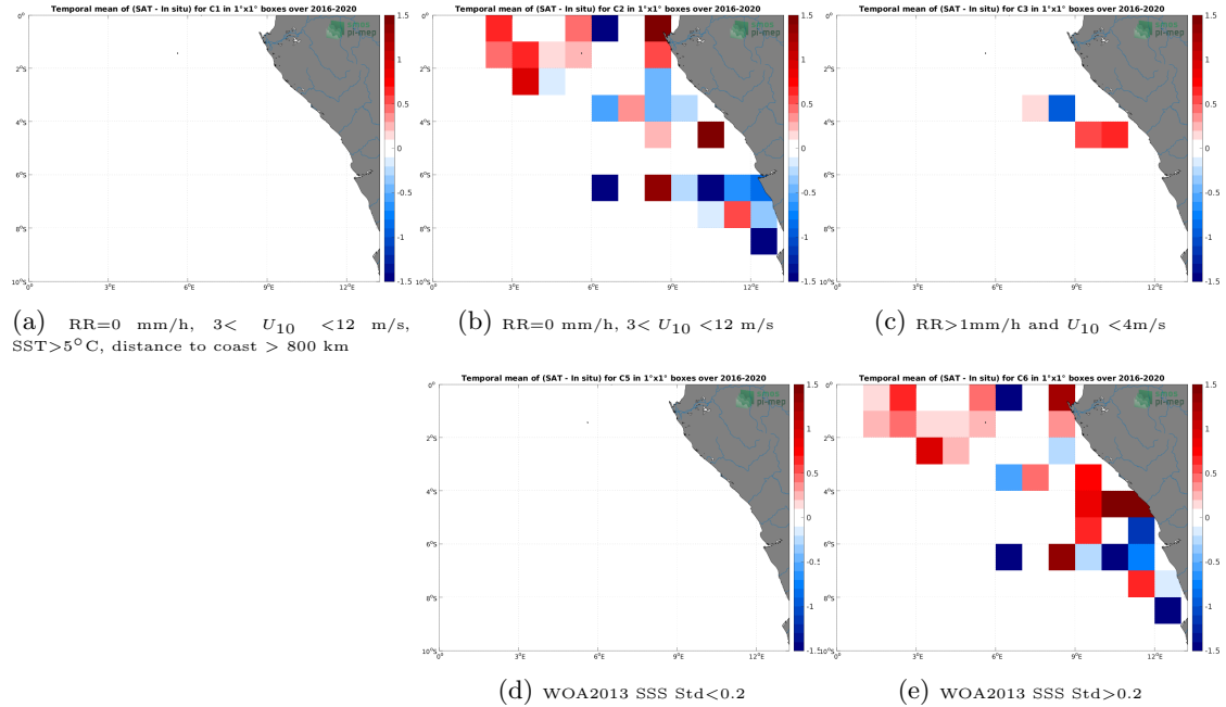
Figure 12: Temporal mean gridded over spatial boxes of size 1^{\circ}\times 1^{\circ} of \Delta\text{SSS} (SMOS SSS L2Q v330 - 0.25 Deg (CATDS-CPDC) - TSG (LEGOS-DM)) for 5 different subdatasets corresponding to:RR=0 mm/h, 3 < U_{10} < 12 m/s, SST >5^{\circ}\text{C} , distance to coast > 800 km (a), RR=0 mm/h, 3 < U_{10} < 12 m/s (b), RR >1 mm/h and U_{10} < 4 m/s (c), WOA2013 SSS Std <0.2 (d), WOA2013 SSS Std >0.2 (e).
