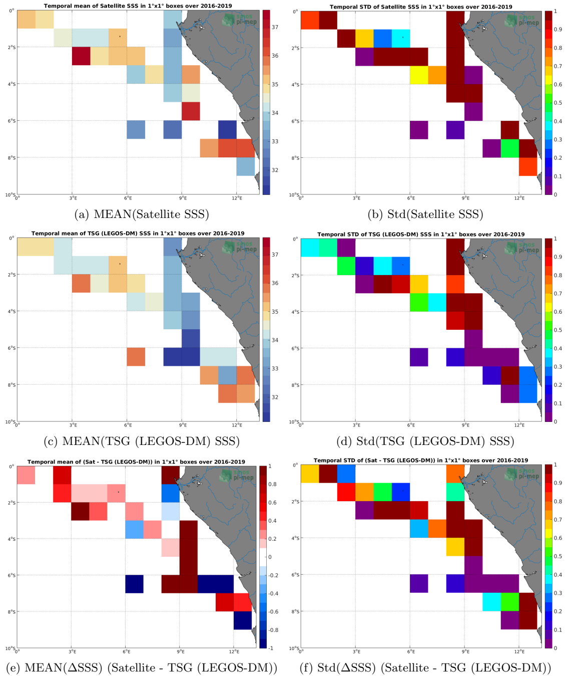
Figure 6: Temporal mean (left) and Std (right) of SSS from SMOS SSS L2Q v330 - 0.25 Deg (CATDS-CPDC) (top), TSG (LEGOS-DM) (middle), and of \Delta SSS (Satellite - TSG (LEGOS-DM)). Only match-up pairs are used to generate these maps.
