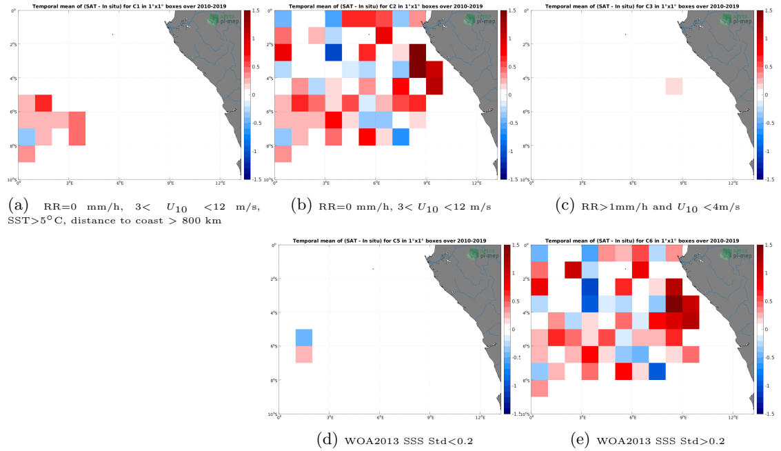
Figure 12: Temporal mean gridded over spatial boxes of size 1^\circ \times 1^\circ of \Delta SSS (SMOS SSS L2Q v330 - 0.25 Deg (CATDS-CPDC) - TSG (GOSUD-Research-vessel)) for 5 different subdatasets corresponding to:RR=0 mm/h, 3 < U_{10} < 12 m/s, SST >5^\circ\text{C} , distance to coast > 800 km (a), RR=0 mm/h, 3 < U_{10} < 12 m/s (b), RR >1 mm/h and U_{10} < 4 m/s (c), WOA2013 SSS Std <0.2 (d), WOA2013 SSS Std >0.2 (e).
