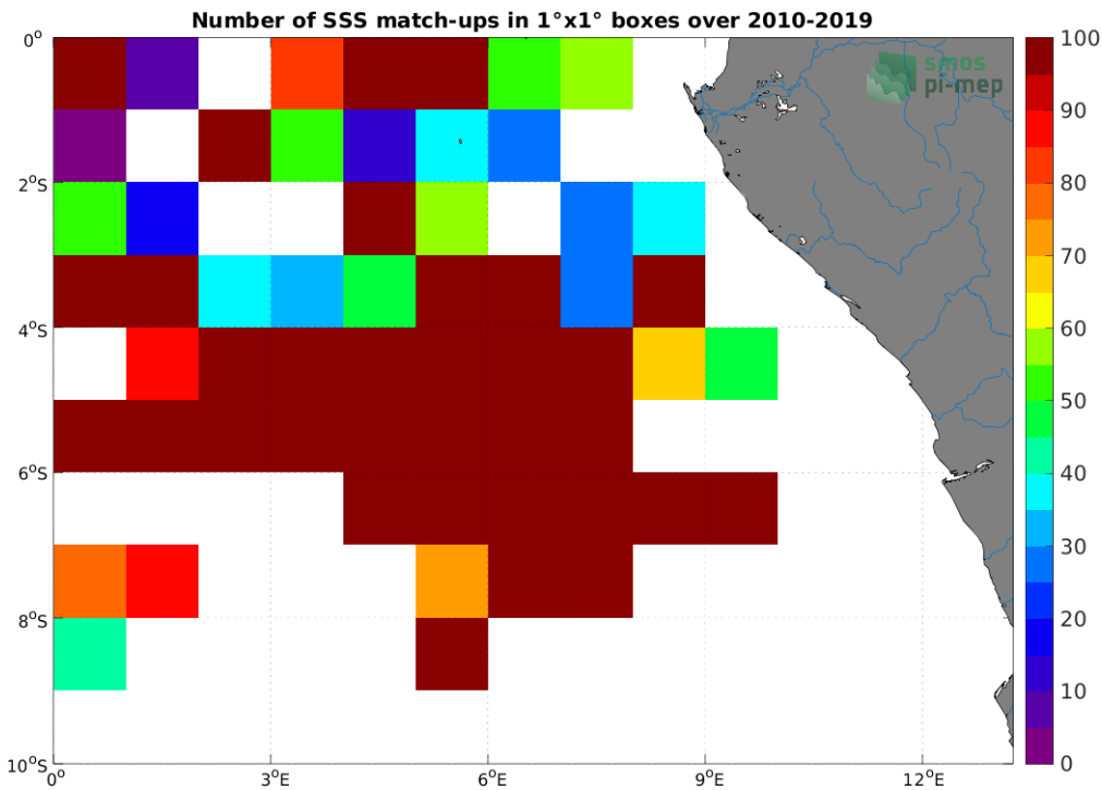
Figure 4: Number of SSS match-ups between TSG (GOSUD-Research-vessel) SSS and the SMOS SSS L2Q v330 - 0.25 Deg (CATDS-CPDC) SSS product for the Congo river plume Pi-MEP region over 1^\circ \times 1^\circ boxes and for the full satellite product period.
