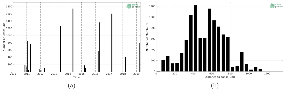
Figure 1: Number of match-ups between TSG (GOSUD-Research-vessel) and SMOS SSS L2Q v330 - 0.25 Deg (CATDS-CPDC) SSS as a function of time (a) and as function of the distance to coast (b) over the Congo river plume Pi-MEP region and for the full satellite product period.
