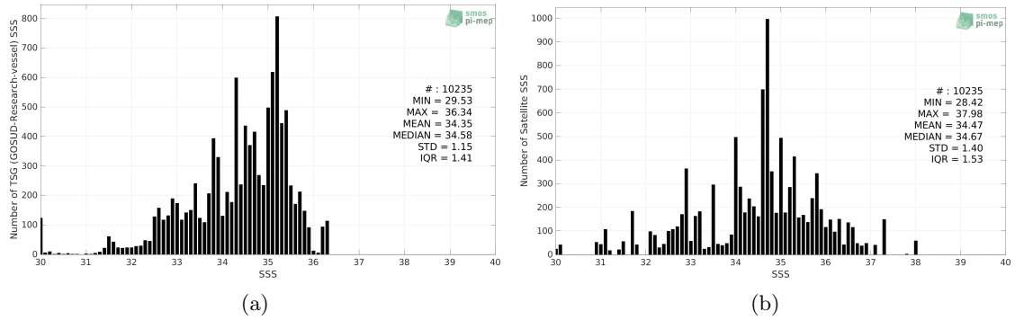
Figure 2: Histograms of SSS from TSG (GOSUD-Research-vessel) (a) and SMOS SSS L2Q v330 - 0.25 Deg (CATDS-CPDC) (b) considering all match-up pairs per bins of 0.1 over the Congo river plume Pi-MEP region and for the full satellite product period.
