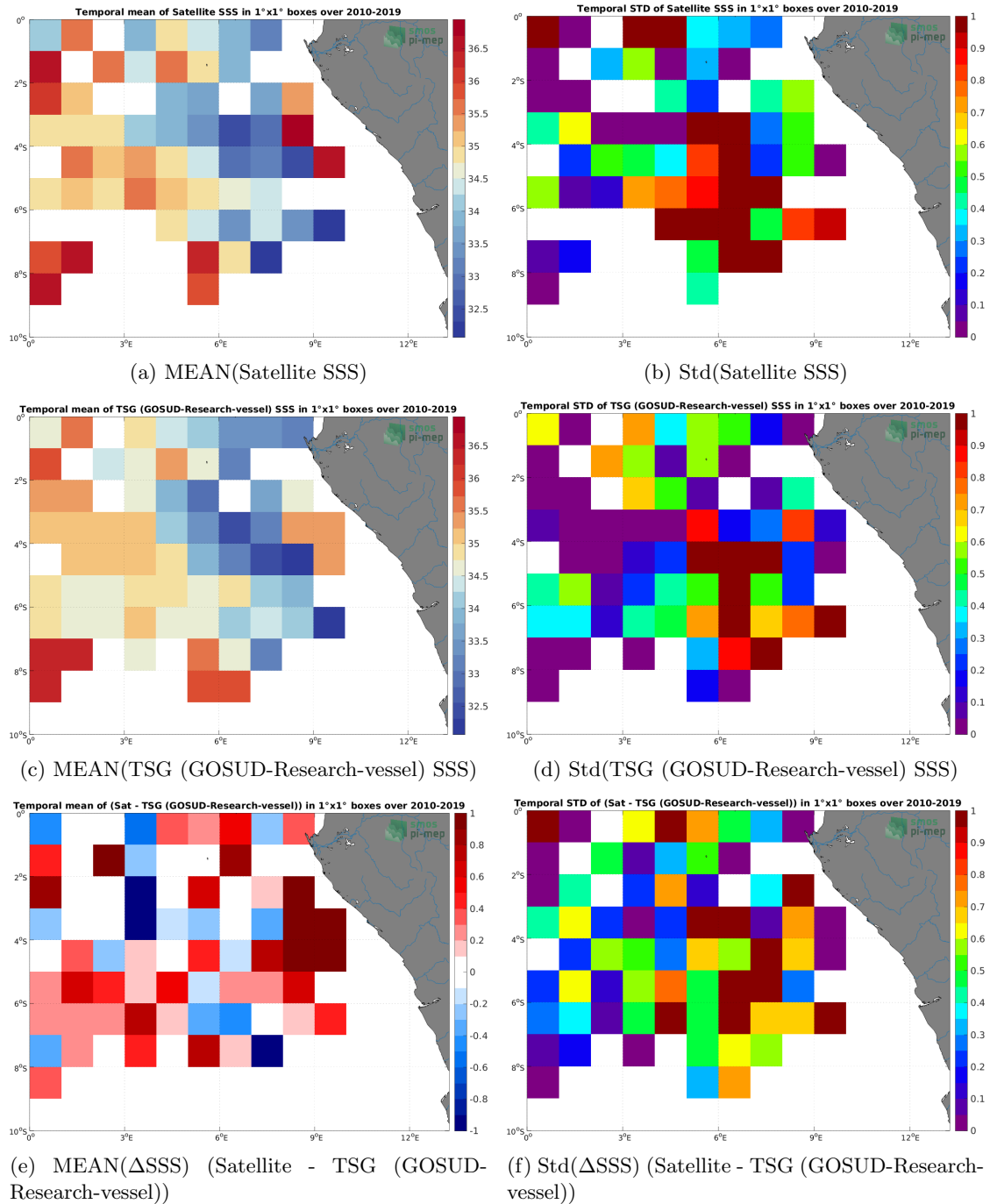
Figure 6: Temporal mean (left) and Std (right) of SSS from SMOS SSS L2Q v330 - 0.25 Deg (CATDS-CPDC) (top), TSG (GOSUD-Research-vessel) (middle), and of \Delta SSS (Satellite - TSG (GOSUD-Research-vessel)). Only match-up pairs are used to generate these maps.
