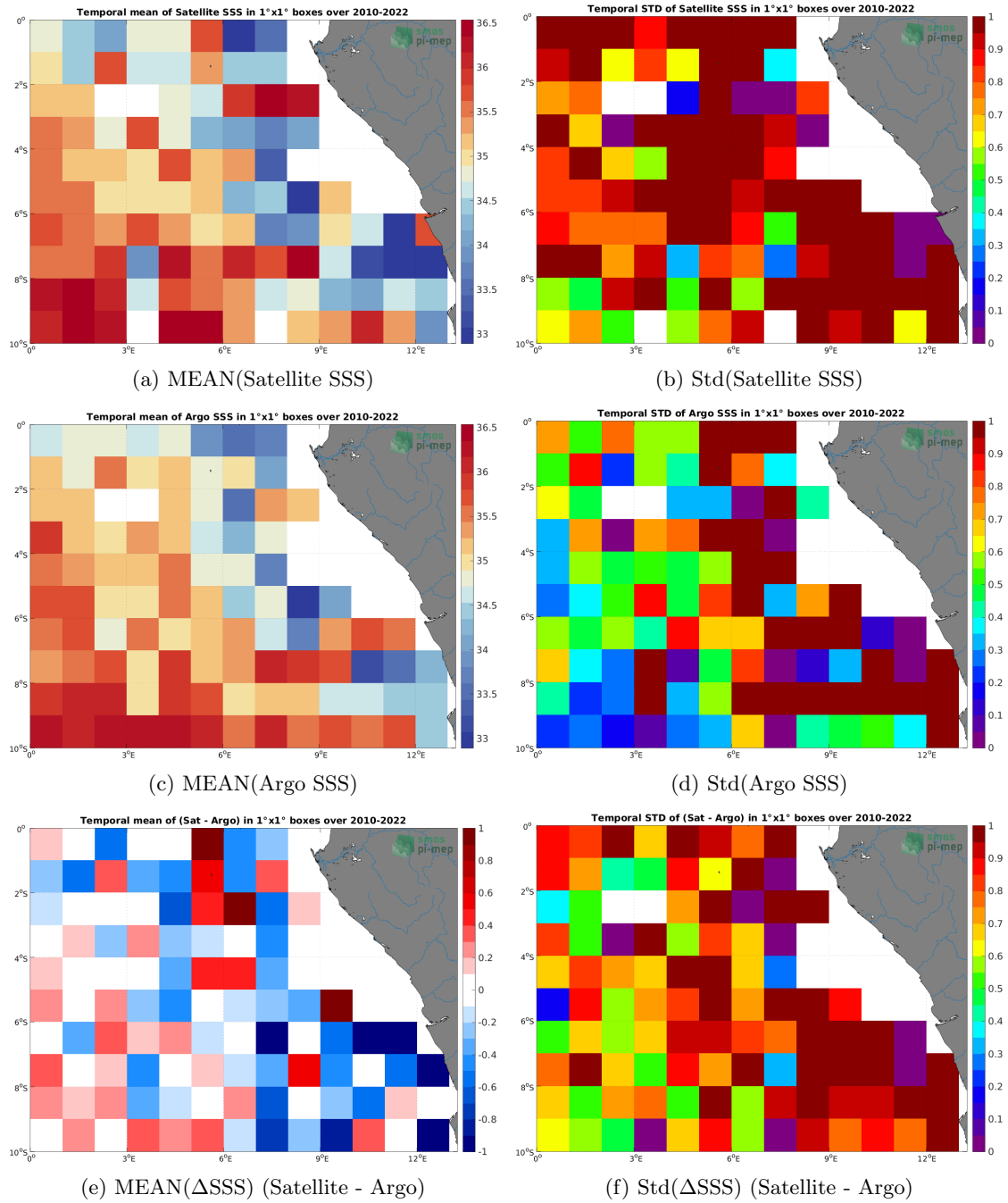
Figure 6: Temporal mean (left) and Std (right) of SSS from SMOS SSS L2Q v330 - 0.25 Deg (CATDS-CPDC) (top), Argo (middle), and of \Delta SSS (Satellite - Argo). Only match-up pairs are used to generate these maps.
