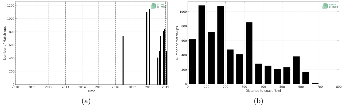
Figure 1: Number of match-ups between TSG (LEGOS-DM) and SMOS SSS L3 v317 - Monthly - 25 km (CATDS-CPDC) SSS as a function of time (a) and as function of the distance to coast (b) over the Congo river plume Pi-MEP region and for the full satellite product period.
