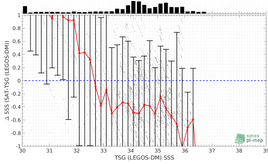
(a) TSG (LEGOS-DM) SSS
