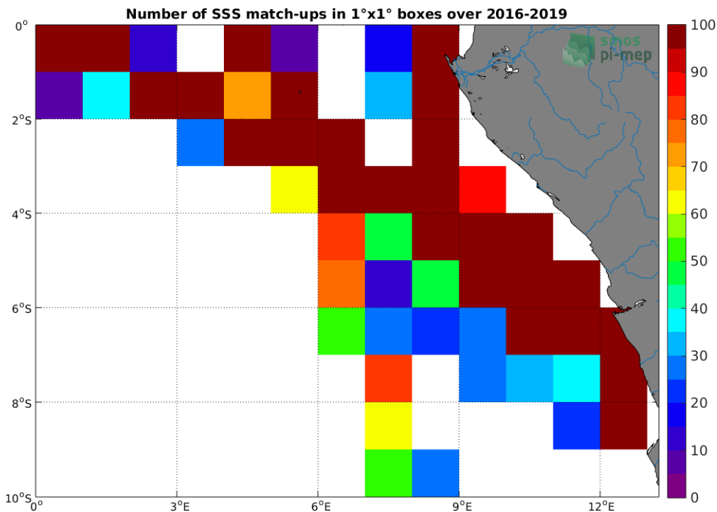
Figure 4: Number of SSS match-ups between TSG (LEGOS-DM) SSS and the SMOS SSS L3 v317 - Monthly - 25 km (CATDS-CPDC) SSS product for the Congo river plume Pi-MEP region over 1°x1° boxes and for the full satellite product period.
