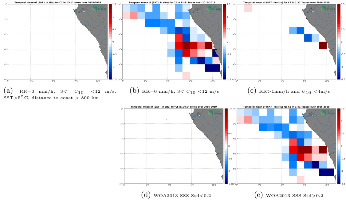
Figure 12: Temporal mean gridded over spatial boxes of size 1^{\circ}\times 1^{\circ} of \Delta\text{SSS} (SMOS SSS L3 v317 - Monthly - 25 km (CATDS-CPDC) - TSG (LEGOS-DM)) for 5 different subdatasets corresponding to:RR=0 mm/h, 3 < U_{10} < 12 m/s, SST > 5^{\circ}\text{C} , distance to coast > 800 km (a), RR=0 mm/h, 3 < U_{10} < 12 m/s (b), RR > 1 mm/h and U_{10} < 4 m/s (c), WOA2013 SSS Std < 0.2 (d), WOA2013 SSS Std > 0.2 (e).
