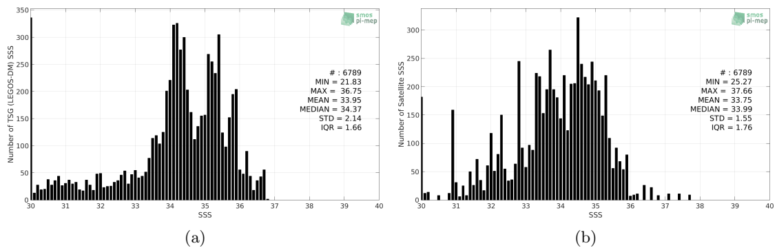
Figure 2: Histograms of SSS from TSG (LEGOS-DM) (a) and SMOS SSS L3 v317 - Monthly - 25 km (CATDS-CPDC) (b) considering all match-up pairs per bins of 0.1 over the Congo river plume Pi-MEP region and for the full satellite product period.
