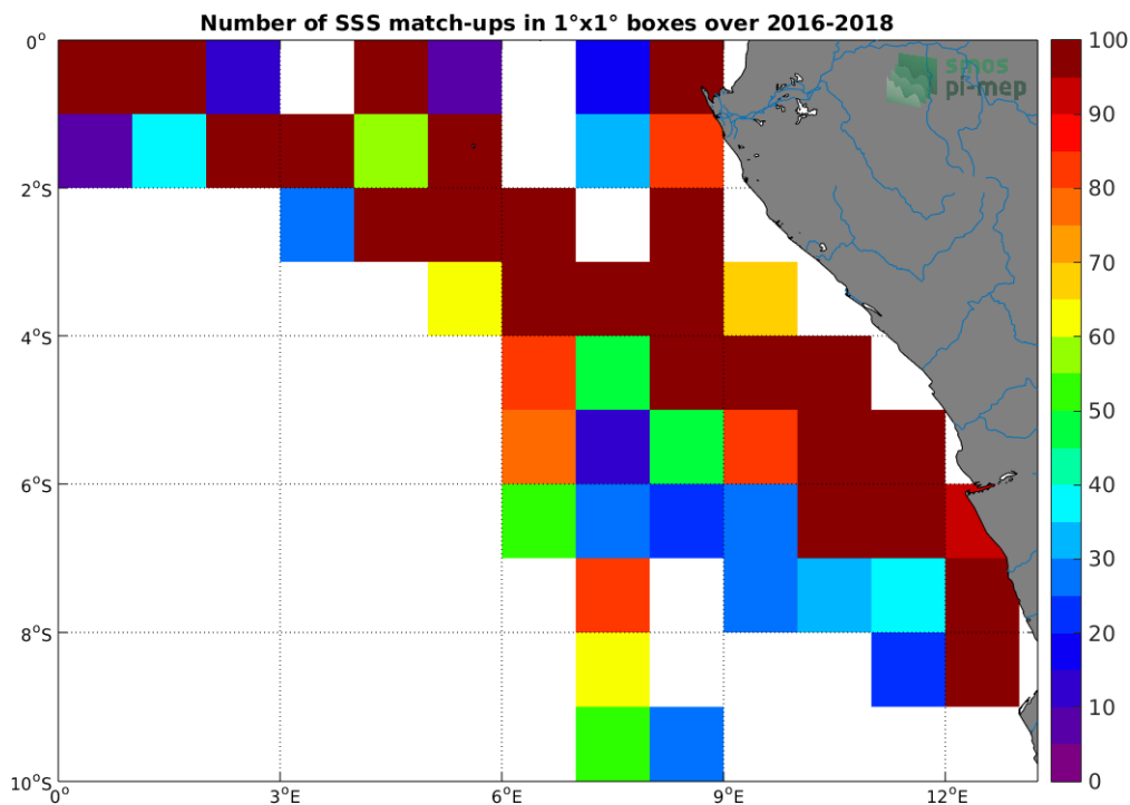
Figure 4: Number of SSS match-ups between TSG-LEGOS-DM SSS and the SMOS-L3-CATDS-CPDC-V317-MONTHLY-25KM SSS product for the Congo river plume Pi-MEP region over 1^\circ \times 1^\circ boxes and for the full satellite product period.
