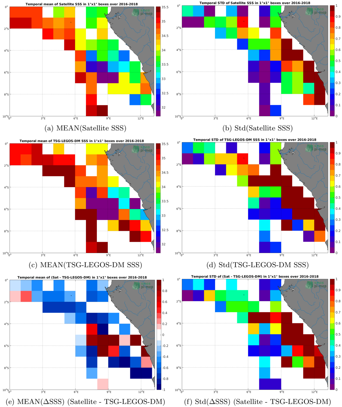
Figure 6: Temporal mean (left) and Std (right) of SSS from SMOS-L3-CATDS-CPDC-V317-MONTHLY-25KM (top), TSG-LEGOS-DM (middle), and of \Delta SSS (Satellite - TSG-LEGOS-DM). Only match-up pairs are used to generate these maps.
