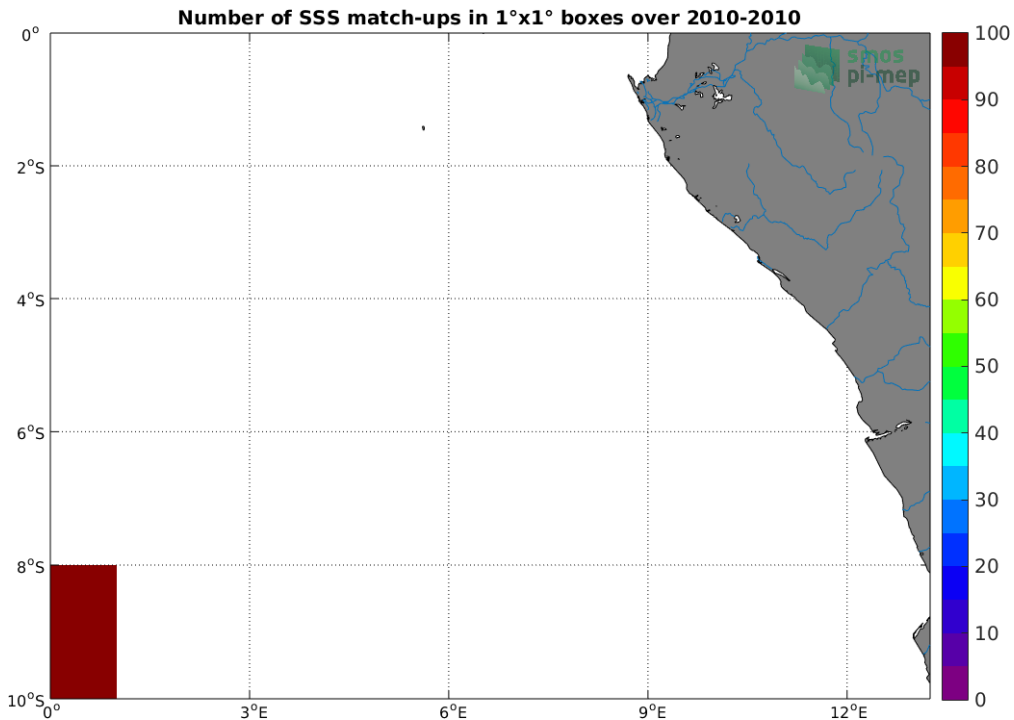
Figure 4: Number of SSS match-ups between TSG (SAMOS) SSS and the SMOS SSS L3 v317 - 10 Days - 25 km (CATDS-CPDC) SSS product for the Congo river plume Pi-MEP region over 1°x1° boxes and for the full satellite product period.
