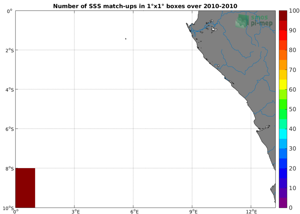
Figure 4: Number of SSS match-ups between TSG-SAMOS SSS and the SMOS L3 v317 - 10 Days - 25 km (CATDS-CPDC) SSS product for the Congo river plume Pi-MEP region over 1^\circ \times 1^\circ boxes and for the full satellite product period.
