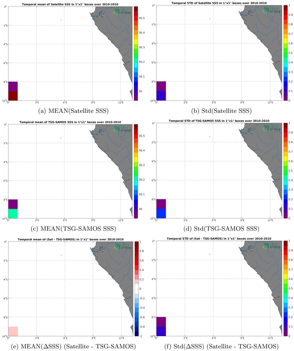
Figure 6: Temporal mean (left) and Std (right) of SSS from SMOS L3 v317 - 10 Days - 25 km (CATDS-CPDC) (top), TSG-SAMOS (middle), and of \Delta SSS (Satellite - TSG-SAMOS). Only match-up pairs are used to generate these maps.
