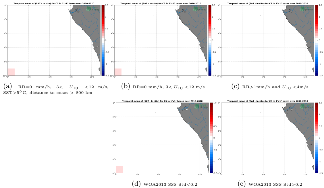
Figure 12: Temporal mean gridded over spatial boxes of size 1^\circ \times 1^\circ of \Delta SSS (SMOS L3 v317 - 10 Days - 25 km (CATDS-CPDC) - TSG-SAMOS) for 5 different subdatasets corresponding to:RR=0 mm/h, 3 < U_{10} < 12 m/s, SST > 5^\circ\text{C} , distance to coast > 800 km (a), RR=0 mm/h, 3 < U_{10} < 12 m/s (b), RR > 1\text{mm/h} and U_{10} < 4\text{m/s} (c), WOA2013 SSS Std < 0.2 (d), WOA2013 SSS Std > 0.2 (e).
