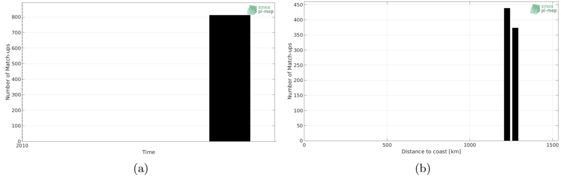
Figure 1: Number of match-ups between TSG-SAMOS and SMOS L3 v317 - 10 Days - 25 km (CATDS-CPDC) SSS as a function of time (a) and as function of the distance to coast (b) over the Congo river plume Pi-MEP region and for the full satellite product period.
