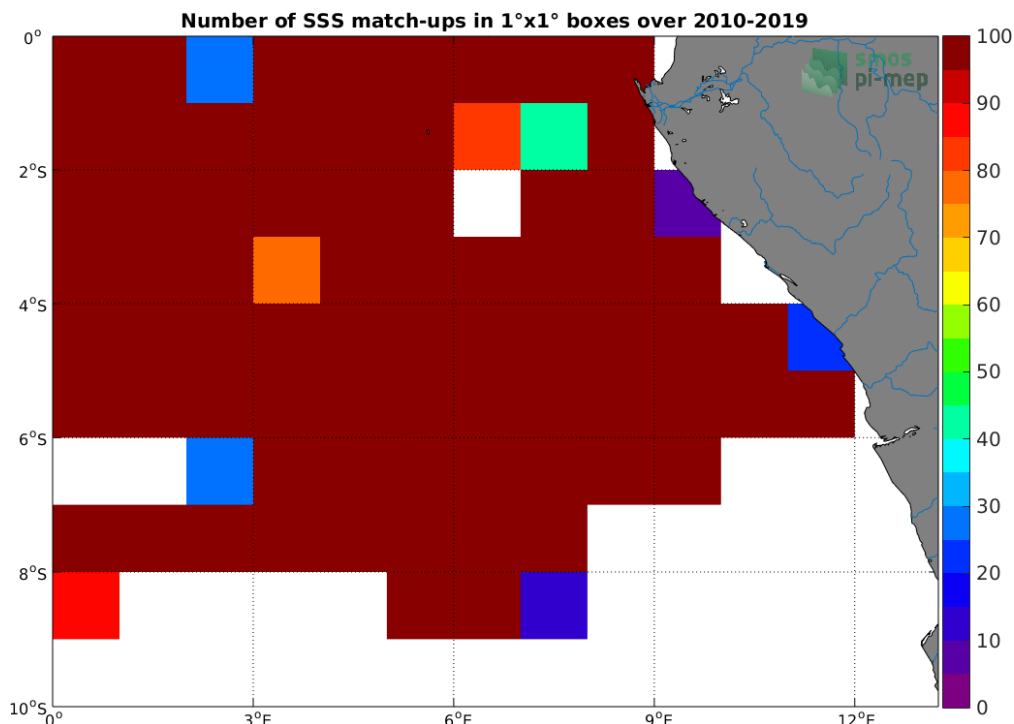
Figure 4: Number of SSS match-ups between TSG (GOSUD-Research-vessel) SSS and the SMOS SSS L3 v317 - 10 Days - 25 km (CATDS-CPDC) SSS product for the Congo river plume Pi-MEP region over 1^\circ \times 1^\circ boxes and for the full satellite product period.
