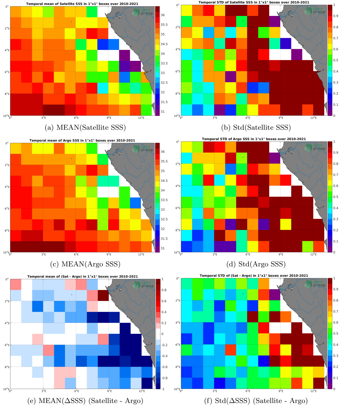
Figure 6: Temporal mean (left) and Std (right) of SSS from SMOS SSS L3 v317 - 10 Days - 25 km (CATDS-CPDC) (top), Argo (middle), and of \Delta SSS (Satellite - Argo). Only match-up pairs are used to generate these maps.
