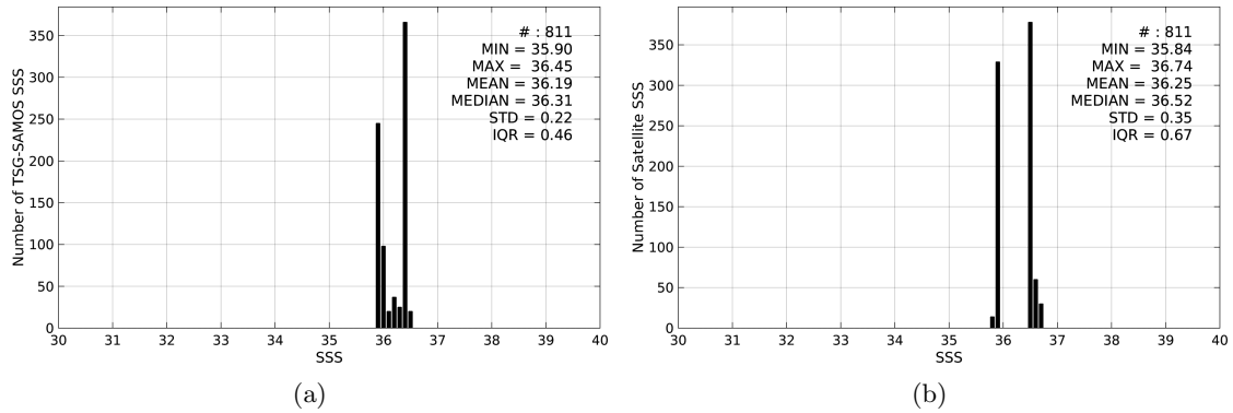
Figure 2: Histograms of SSS from TSG-SAMOS (a) and SMOS-L3-CATDS-CPDC-V3-MONTHLY-25KM (b) considering all match-up pairs per bins of 0.1 over the Congo river plume Pi-MEP region and for the full satellite product period.
