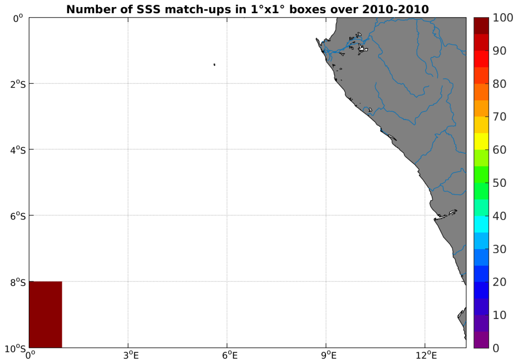
Figure 4: Number of SSS match-ups between TSG-SAMOS SSS and the SMOS-L3-CATDS-CPDC-V3-MONTHLY-25KM SSS product for the Congo river plume Pi-MEP region over 1°x1° boxes and for the full satellite product period.
