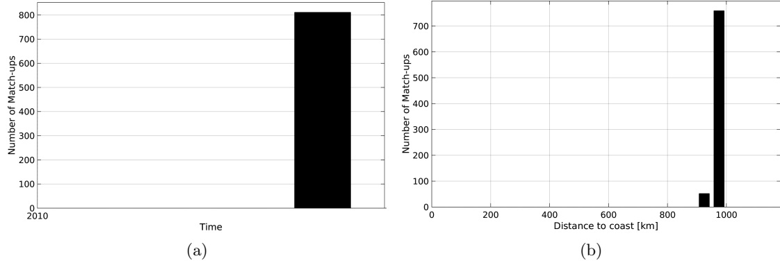
Figure 1: Number of match-ups between TSG-SAMOS and SMOS-L3-CATDS-CPDC-V3-MONTHLY-25KM SSS as a function of time (a) and as function of the distance to coast (b) over the Congo river plume Pi-MEP region and for the full satellite product period.
