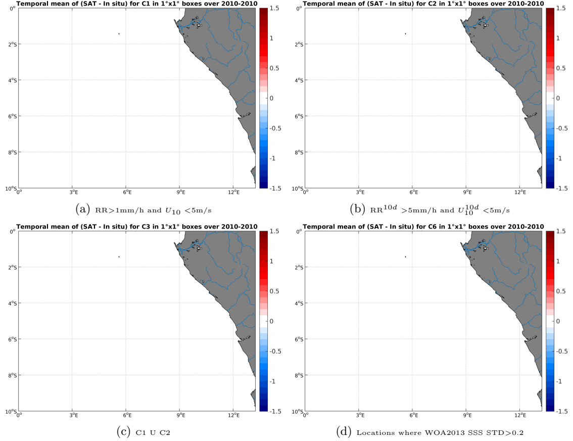
Figure 12: Temporal mean gridded over spatial boxes of size 1^\circ \times 1^\circ of \Delta SSS (SMOS-L3-CATDS-CPDC-V3-MONTHLY-25KM - TSG-SAMOS) for 4 different subdatasets corresponding to: RR > 1 mm/h and U_{10} < 5 m/s (a), RR^{10d} > 5 mm/h and U_{10}^{10d} < 5 m/s (b), C1 U C2 (c), Locations where WOA2013 SSS STD > 0.2 (d).
