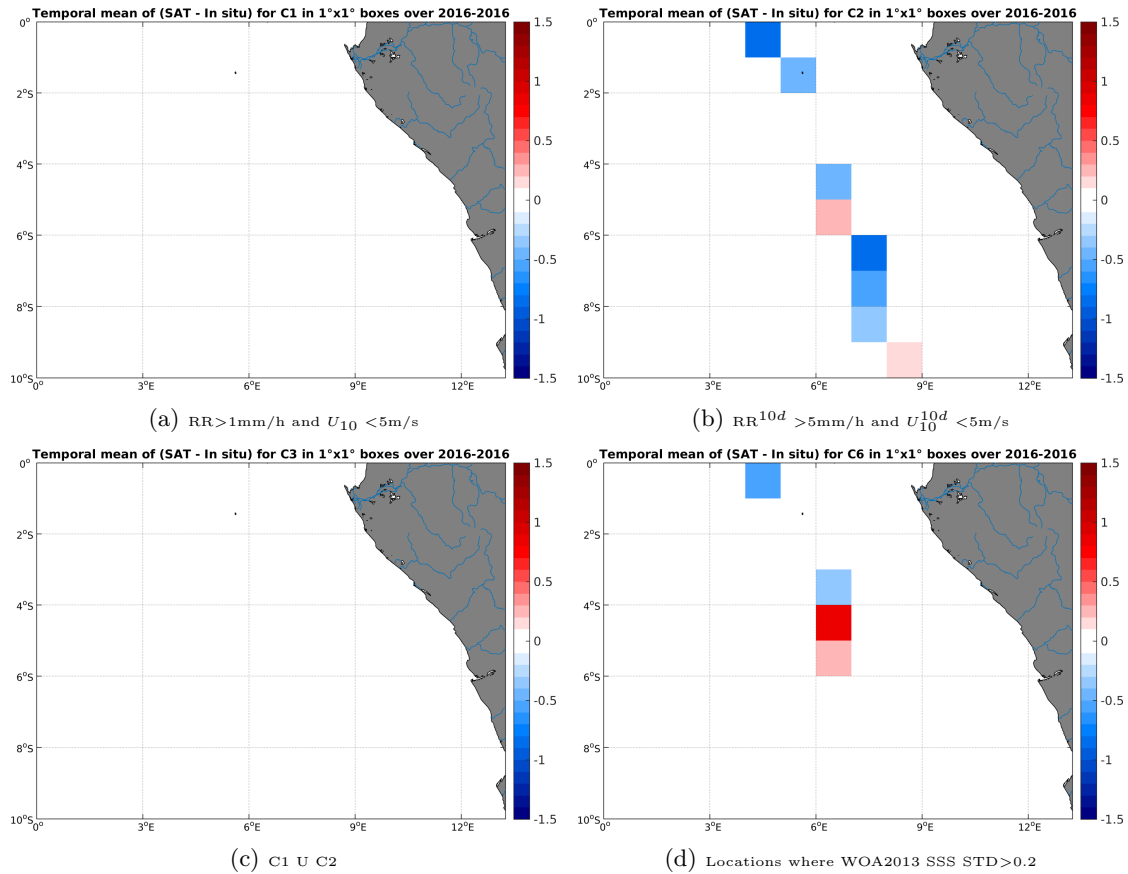
Figure 12: Temporal mean gridded over spatial boxes of size 1^\circ \times 1^\circ of \Delta SSS (SMOS-L3-CATDS-CPDC-V3-MONTHLY-25KM - TSG-LEGOS-DM) for 4 different subdatasets corresponding to: RR > 1 mm/h and U_{10} < 5 m/s (a), RR^{10d} > 5 mm/h and U_{10}^{10d} < 5 m/s (b), C1 \cup C2 (c), Locations where WOA2013 SSS STD > 0.2 (d).
