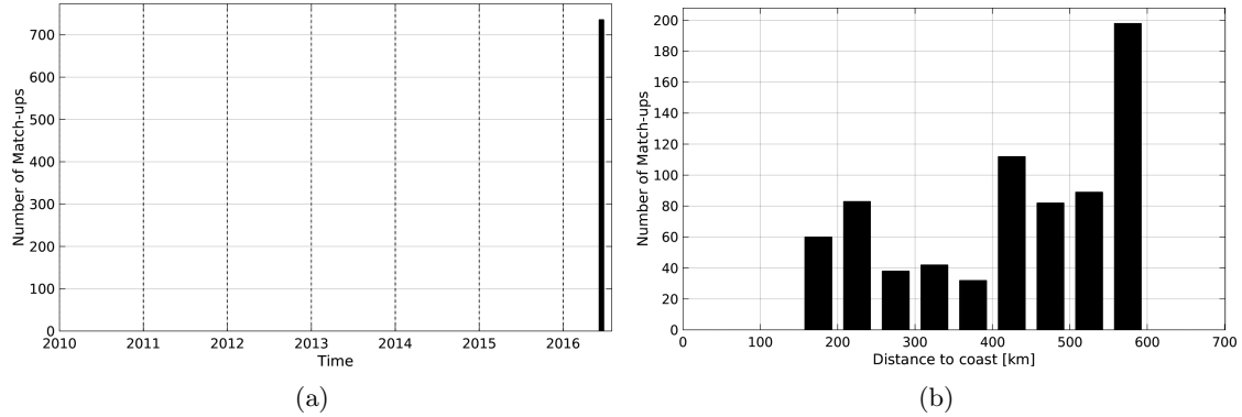
Figure 1: Number of match-ups between TSG-LEGOS-DM and SMOS-L3-CATDS-CPDC-V3-MONTHLY-25KM SSS as a function of time (a) and as function of the distance to coast (b) over the Congo river plume Pi-MEP region and for the full satellite product period.
