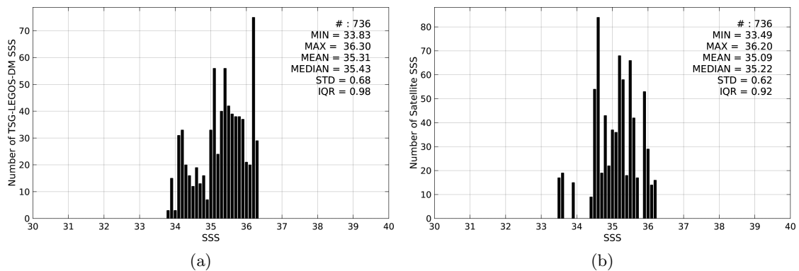
Figure 2: Histograms of SSS from TSG-LEGOS-DM (a) and SMOS-L3-CATDS-CPDC-V3-MONTHLY-25KM (b) considering all match-up pairs per bins of 0.1 over the Congo river plume Pi-MEP region and for the full satellite product period.
