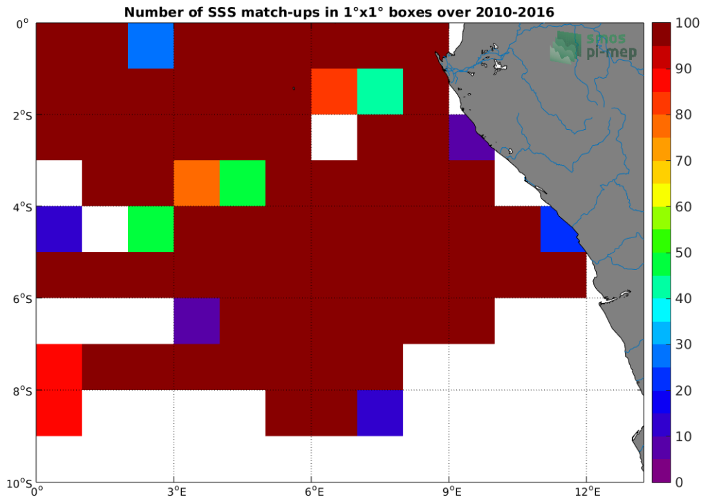
Figure 4: Number of SSS match-ups between TSG-GOSUD-Research-vessel SSS and the SMOS-L3-CATDS-CPDC-V3-MONTHLY-25KM SSS product for the Congo river plume Pi-MEP region over 1°x1° boxes and for the full satellite product period.
