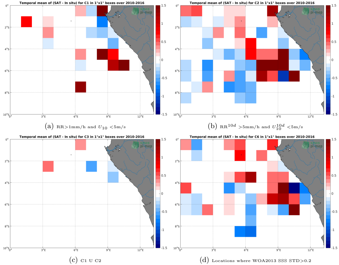
Figure 12: Temporal mean gridded over spatial boxes of size 1^\circ \times 1^\circ of \Delta SSS (SMOS-L3-CATDS-CPDC-V3-MONTHLY-25KM - TSG-GOSUD-Research-vessel) for 4 different subdatasets corresponding to: RR > 1\text{mm/h} and U_{10} < 5\text{m/s} (a), RR^{10d} > 5\text{mm/h} and U_{10}^{10d} < 5\text{m/s} (b), C1 \cup C2 (c), Locations where WOA2013 SSS STD > 0.2 (d).
