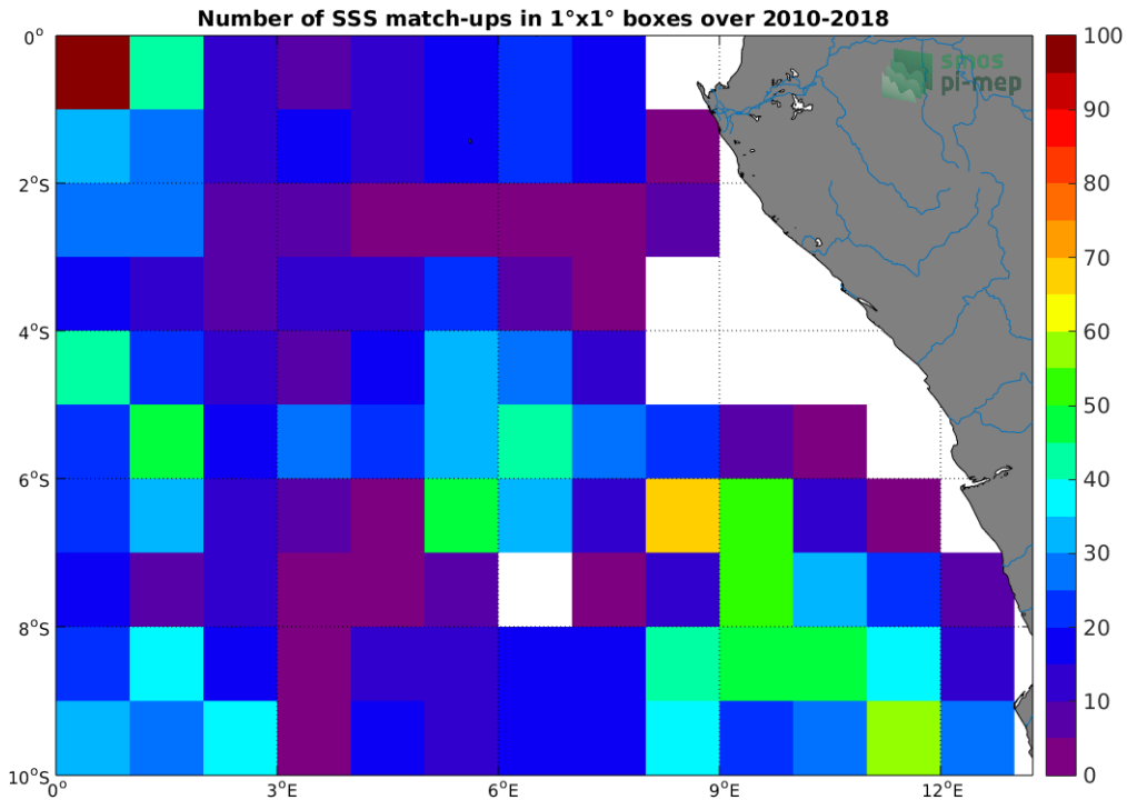
Figure 4: Number of SSS match-ups between Argo SSS and the SMOS-L3-CATDS-CPDC-V3-MONTHLY-25KM SSS product for the Congo river plume Pi-MEP region over 1°x1° boxes and for the full satellite product period.
