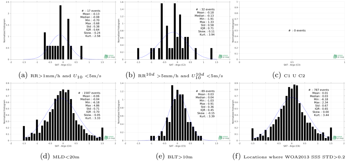
Figure 13: Normalized histogram of \Delta SSS (SMOS-L3-CATDS-CPDC-V3-MONTHLY-25KM - Argo) for 6 different subdatasets corresponding to: RR > 1mm/h and U_{10} < 5 m/s (a), RR 10d > 5mm/h and U_{10}^{10d} < 5 m/s (b), C1 U C2 (c), MLD < 20m (d), BLT > 10m (e), Locations where WOA2013 SSS STD > 0.2 (f).
