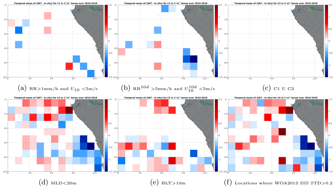
Figure 12: Temporal mean gridded over spatial boxes of size 1^\circ \times 1^\circ of \Delta\text{SSS} (SMOS-L3-CATDS-CPDC-V3-MONTHLY-25KM - Argo) for 6 different subdatasets corresponding to: RR > 1\text{mm/h} and U_{10} < 5\text{m/s} (a), RR^{10d} > 5\text{mm/h} and U_{10}^{10d} < 5\text{m/s} (b), C1 U C2 (c), MLD < 20\text{m} (d), BLT > 10\text{m} (e), Locations where WOA2013 SSS STD > 0.2 (f).
