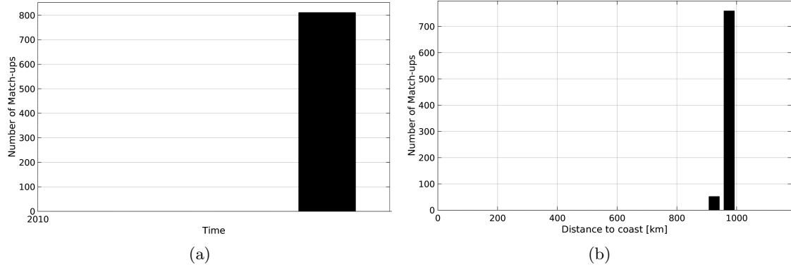
Figure 1: Number of match-ups between TSG-SAMOS and SMOS-L3-CATDS-CPDC-V3-10DAYS-25KM SSS as a function of time (a) and as function of the distance to coast (b) over the Congo river plume Pi-MEP region and for the full satellite product period.
