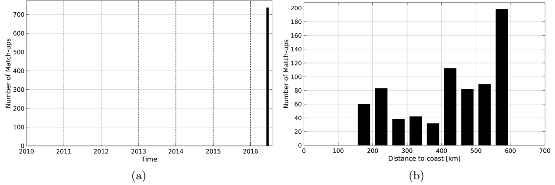
Figure 1: Number of match-ups between TSG-LEGOS-DM and SMOS-L3-CATDS-CPDC-V3-10DAYS-25KM SSS as a function of time (a) and as function of the distance to coast (b) over the Congo river plume Pi-MEP region and for the full satellite product period.
