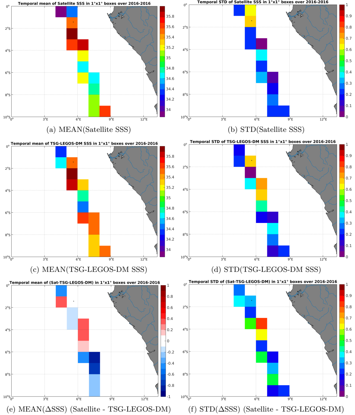
Figure 6: Temporal mean (left) and STD (right) of SSS from SMOS-L3-CATDS-CPDC-V3-10DAYS-25KM (top), TSG-LEGOS-DM (middle), and of ΔSSS (Satellite - TSG-LEGOS-DM). Only match-up pairs are used to generate these maps.
