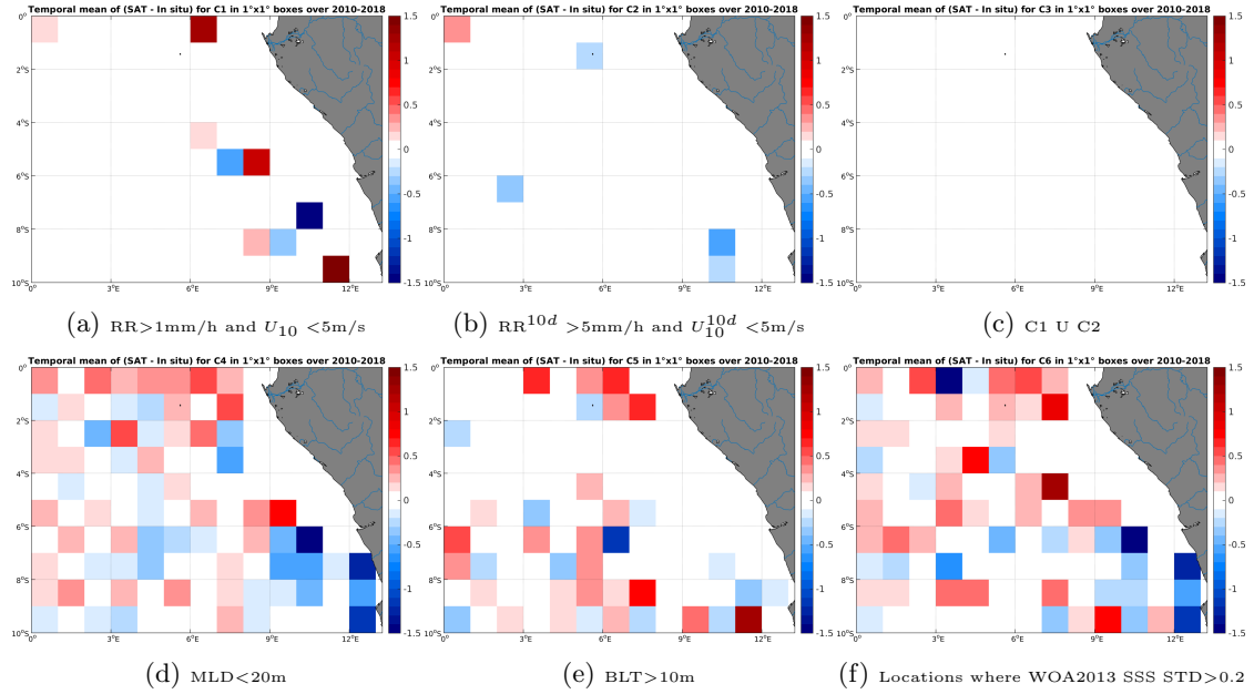
Figure 12: Temporal mean gridded over spatial boxes of size 1^\circ \times 1^\circ of \Delta SSS (SMOS-L3-CATDS-CPDC-V3-10DAYS-25KM - Argo) for 6 different subdatasets corresponding to: RR > 1\text{mm/h} and U_{10} < 5\text{m/s} (a), RR^{10d} > 5\text{mm/h} and U_{10}^{10d} < 5\text{m/s} (b), C1 U C2 (c), MLD < 20\text{m} (d), BLT > 10\text{m} (e), Locations where WOA2013 SSS STD > 0.2 (f).
