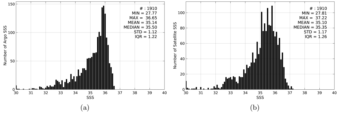
Figure 2: Histograms of SSS from Argos (a) and SMOS-L3-CATDS-CPDC-V3-10DAYS-25KM (b) considering all match-up pairs per bins of 0.1 over the Congo river plume Pi-MEP region and for the full satellite product period.
