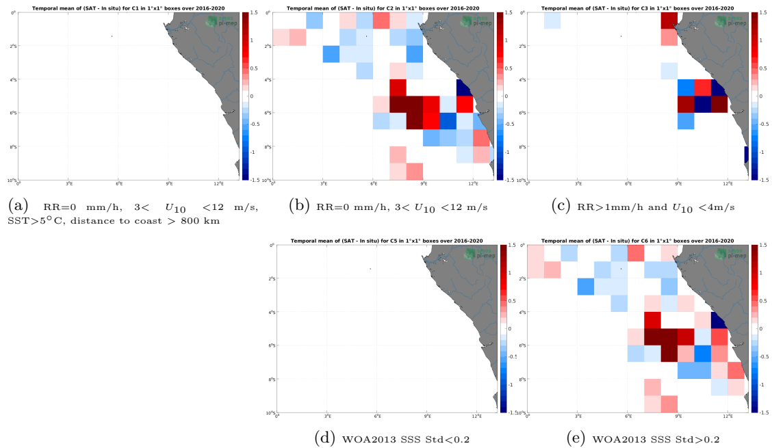
Figure 12: Temporal mean gridded over spatial boxes of size 1^\circ \times 1^\circ of \Delta SSS (SMOS SSS L3 v2 - 9-Days (BEC) - TSG (LEGOS-DM)) for 5 different subdatasets corresponding to:RR=0 mm/h, 3 < U_{10} < 12 m/s, SST > 5^\circ\text{C} , distance to coast > 800 km (a), RR=0 mm/h, 3 < U_{10} < 12 m/s (b), RR > 1 mm/h and U_{10} < 4 m/s (c), WOA2013 SSS Std < 0.2 (d), WOA2013 SSS Std > 0.2 (e).
