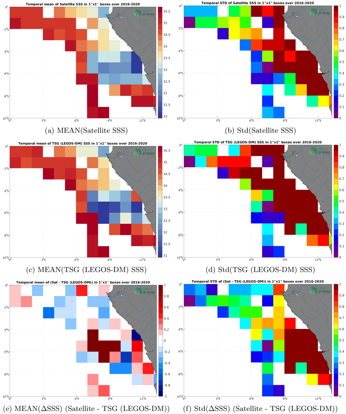
Figure 6: Temporal mean (left) and Std (right) of SSS from SMOS SSS L3 v2 - 9-Days (BEC) (top), TSG (LEGOS-DM) (middle), and of \Delta SSS (Satellite - TSG (LEGOS-DM)). Only match-up pairs are used to generate these maps.
