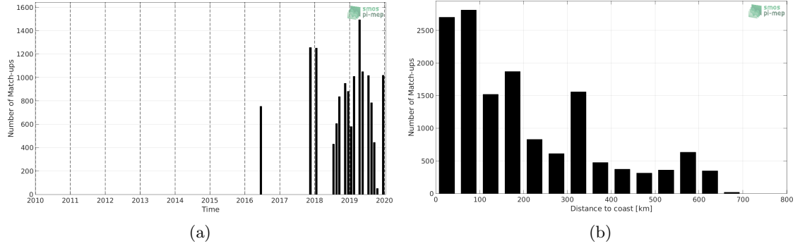
Figure 1: Number of match-ups between TSG (LEGOS-DM) and SMOS SSS L3 v2 - 9-Days (BEC) SSS as a function of time (a) and as function of the distance to coast (b) over the Congo river plume Pi-MEP region and for the full satellite product period.
