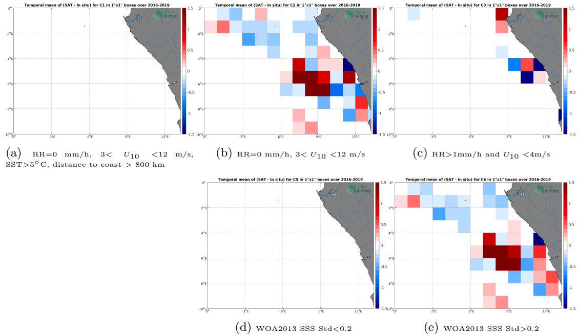
Figure 12: Temporal mean gridded over spatial boxes of size 1^\circ \times 1^\circ of \Delta SSS (SMOS SSS L3 v2 - 9-Days (BEC) - TSG (LEGOS-DM)) for 5 different subdatasets corresponding to: RR=0 mm/h, 3 < U_{10} < 12 m/s, SST > 5^\circ C , distance to coast > 800 km (a), RR=0 mm/h, 3 < U_{10} < 12 m/s (b), RR > 1 mm/h and U_{10} < 4 m/s (c), WOA2013 SSS Std < 0.2 (d), WOA2013 SSS Std > 0.2 (e).
