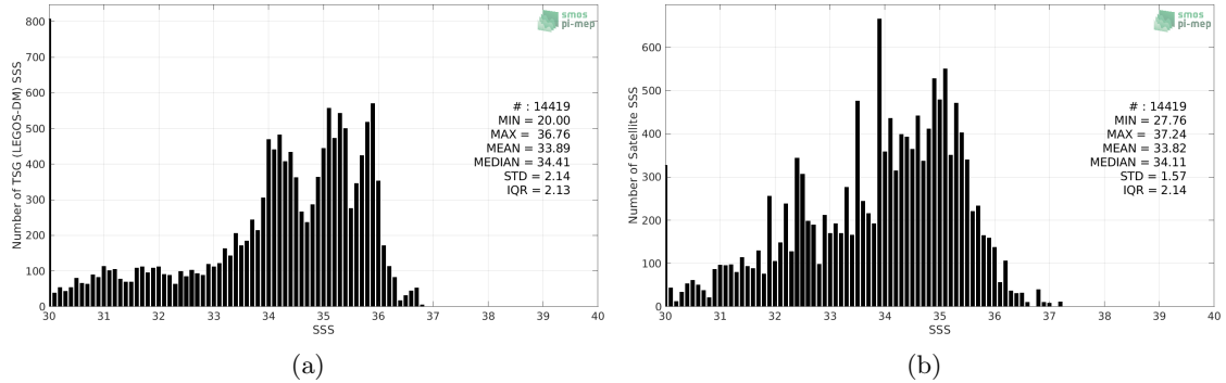
Figure 2: Histograms of SSS from TSG (LEGOS-DM) (a) and SMOS SSS L3 v2 - 9-Days (BEC) (b) considering all match-up pairs per bins of 0.1 over the Congo river plume Pi-MEP region and for the full satellite product period.
