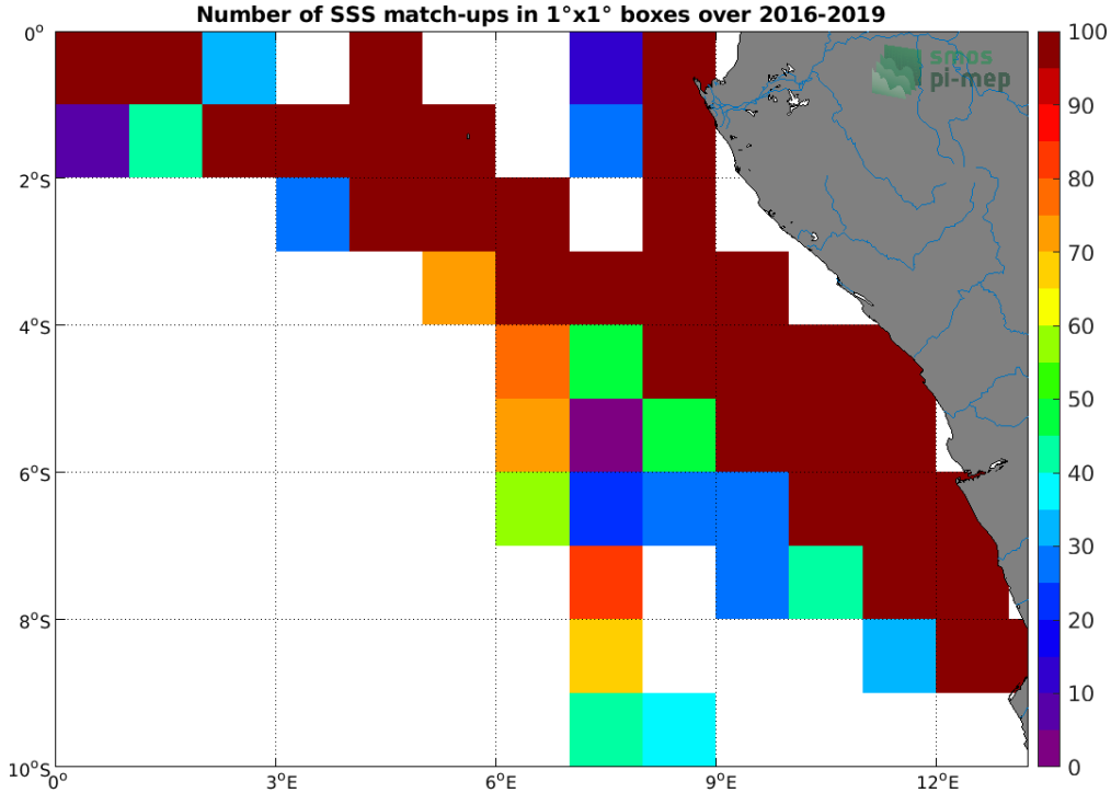
Figure 4: Number of SSS match-ups between TSG (LEGOS-DM) SSS and the SMOS SSS L3 v2 - 9-Days (BEC) SSS product for the Congo river plume Pi-MEP region over 1^\circ \times 1^\circ boxes and for the full satellite product period.
