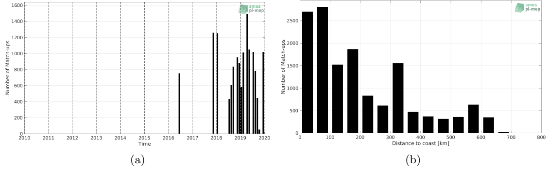
Figure 1: Number of match-ups between TSG (LEGOS-DM) and SMOS SSS L3 v2 - 9-Days (BEC) SSS as a function of time (a) and as function of the distance to coast (b) over the Congo river plume Pi-MEP region and for the full satellite product period.
