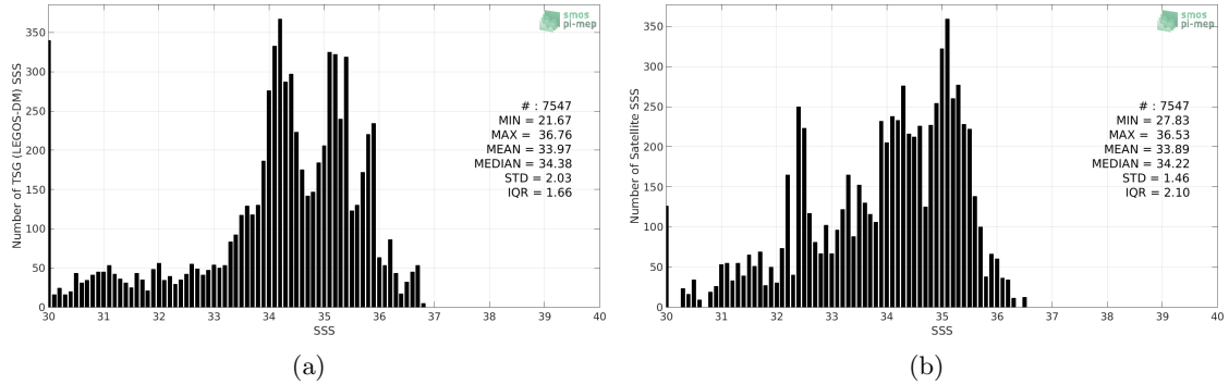
Figure 2: Histograms of SSS from TSG (LEGOS-DM) (a) and SMOS L3 v2 - 9-Days (BEC) (b) considering all match-up pairs per bins of 0.1 over the Congo river plume Pi-MEP region and for the full satellite product period.
