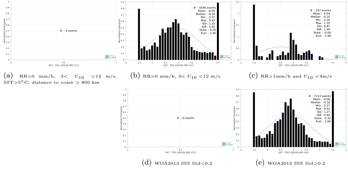
Figure 13: Normalized histogram of \Delta\text{SSS} (SMOS L3 v2 - 9-Days (BEC) - TSG (LEGOS-DM)) for 5 different subdatasets corresponding to: RR=0 mm/h, 3 < U_{10} < 12 m/s, SST > 5^\circ\text{C} , distance to coast > 800 km (a), RR=0 mm/h, 3 < U_{10} < 12 m/s (b), RR > 1 mm/h and U_{10} < 4 m/s (c), WOA2013 SSS Std < 0.2 (d), WOA2013 SSS Std > 0.2 (e).
