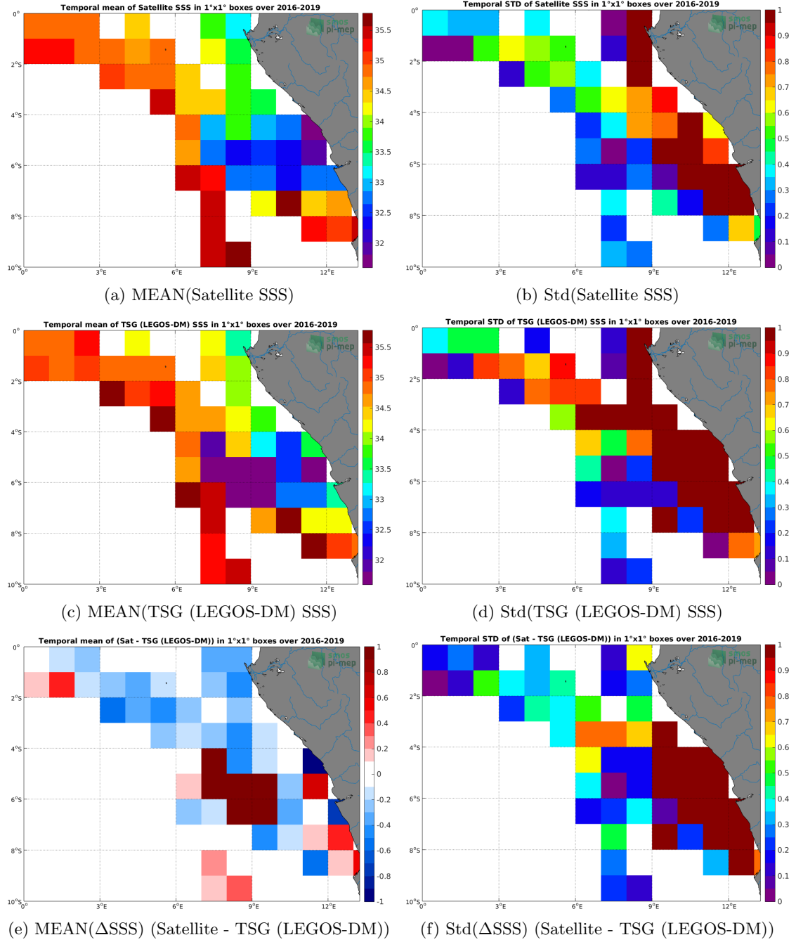
Figure 6: Temporal mean (left) and Std (right) of SSS from SMOS L3 v2-9-Days (BEC) (top), TSG (LEGOS-DM) (middle), and of \Delta SSS (Satellite - TSG (LEGOS-DM)). Only match-up pairs are used to generate these maps.
