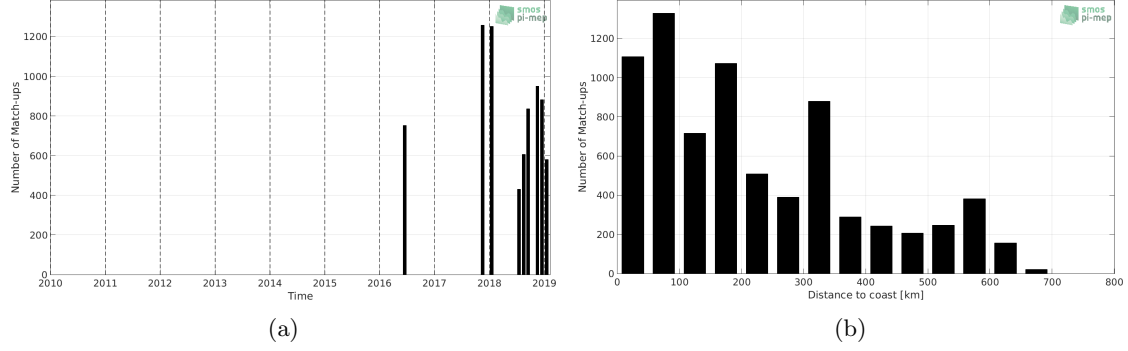
Figure 1: Number of match-ups between TSG (LEGOS-DM) and SMOS L3 v2 - 9-Days (BEC) SSS as a function of time (a) and as function of the distance to coast (b) over the Congo river plume Pi-MEP region and for the full satellite product period.
