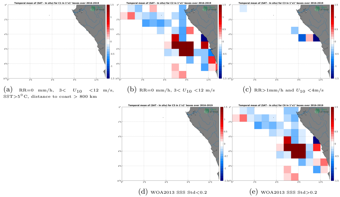
Figure 12: Temporal mean gridded over spatial boxes of size 1^\circ \times 1^\circ of \Delta SSS (SMOS L3 v2 - 9-Days (BEC) - TSG (LEGOS-DM)) for 5 different subdatasets corresponding to: RR=0 mm/h, 3 < U_{10} < 12 m/s, SST > 5^\circ C , distance to coast > 800 km (a), RR=0 mm/h, 3 < U_{10} < 12 m/s (b), RR > 1 mm/h and U_{10} < 4 m/s (c), WOA2013 SSS Std < 0.2 (d), WOA2013 SSS Std > 0.2 (e).
