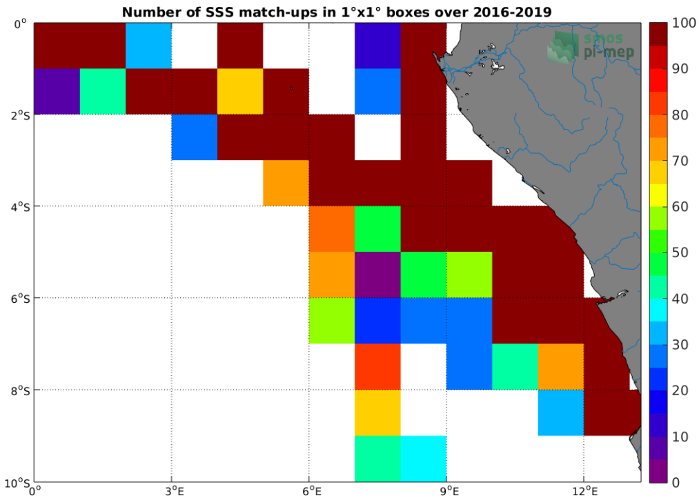
Figure 4: Number of SSS match-ups between TSG (LEGOS-DM) SSS and the SMOS L3 v2 - 9-Days (BEC) SSS product for the Congo river plume Pi-MEP region over 1°x1° boxes and for the full satellite product period.
