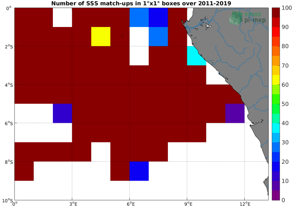
Figure 4: Number of SSS match-ups between TSG (GOSUD-Research-vessel) SSS and the SMOS SSS L3 v2 - 9-Days (BEC) SSS product for the Congo river plume Pi-MEP region over 1^\circ \times 1^\circ boxes and for the full satellite product period.
