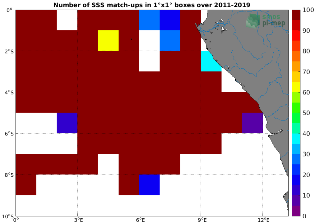
Figure 4: Number of SSS match-ups between TSG (GOSUD-Research-vessel) SSS and the SMOS SSS L3 v2 - 9-Days (BEC) SSS product for the Congo river plume Pi-MEP region over 1°x1° boxes and for the full satellite product period.
