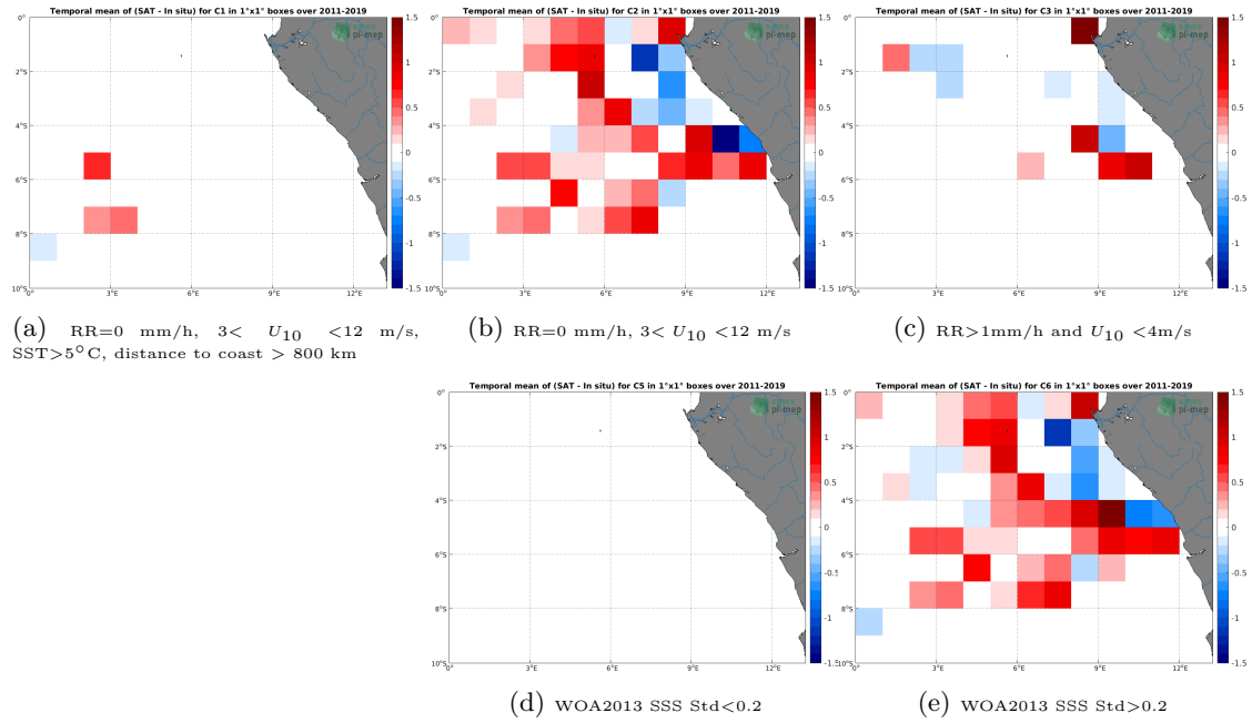
Figure 12: Temporal mean gridded over spatial boxes of size 1^\circ \times 1^\circ of \Delta SSS (SMOS SSS L3 v2 - 9-Days (BEC) - TSG (GOSUD-Research-vessel)) for 5 different subdatasets corresponding to: RR=0 mm/h, 3 < U_{10} < 12 m/s, SST >5^\circ\text{C} , distance to coast > 800 km (a), RR=0 mm/h, 3 < U_{10} < 12 m/s (b), RR >1 mm/h and U_{10} < 4 m/s (c), WOA2013 SSS Std <0.2 (d), WOA2013 SSS Std >0.2 (e).
