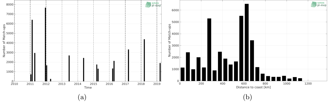
Figure 1: Number of match-ups between TSG (GOSUD-Research-vessel) and SMOS SSS L3 v2 - 9-Days (BEC) SSS as a function of time (a) and as function of the distance to coast (b) over the Congo river plume Pi-MEP region and for the full satellite product period.
