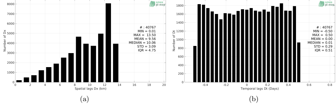
Figure 5: Histograms of the spatial (a) and temporal (b) lags between the time of the TSG (GOSUD-Research-vessel) measurements and the date of the corresponding SMOS SSS L3 v2 - 9-Days (BEC) SSS product.
