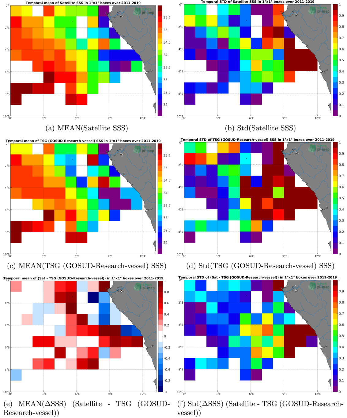
Figure 6: Temporal mean (left) and Std (right) of SSS from SMOS SSS L3 v2 - 9-Days (BEC) (top), TSG (GOSUD-Research-vessel) (middle), and of \Delta SSS (Satellite - TSG (GOSUD-Research-vessel)). Only match-up pairs are used to generate these maps.
