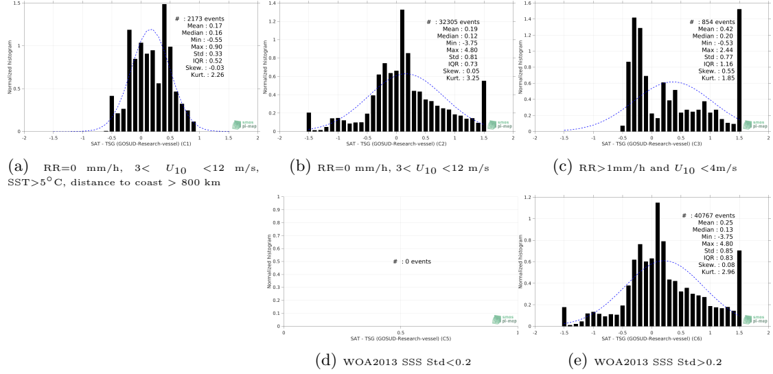
Figure 13: Normalized histogram of \Delta SSS (SMOS SSS L3 v2 - 9-Days (BEC) - TSG (GOSUD-Research-vessel)) for 5 different subdatasets corresponding to: RR=0 mm/h, 3 < U_{10} < 12 m/s, SST>5°C, distance to coast > 800 km (a), RR=0 mm/h, 3 < U_{10} < 12 m/s (b), RR>1mm/h and U_{10} < 4 m/s (c), WOA2013 SSS Std<0.2 (d), WOA2013 SSS Std>0.2 (e).
