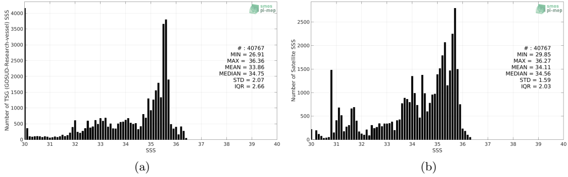
Figure 2: Histograms of SSS from TSG (GOSUD-Research-vessel) (a) and SMOS SSS L3 v2 - 9-Days (BEC) (b) considering all match-up pairs per bins of 0.1 over the Congo river plume Pi-MEP region and for the full satellite product period.
