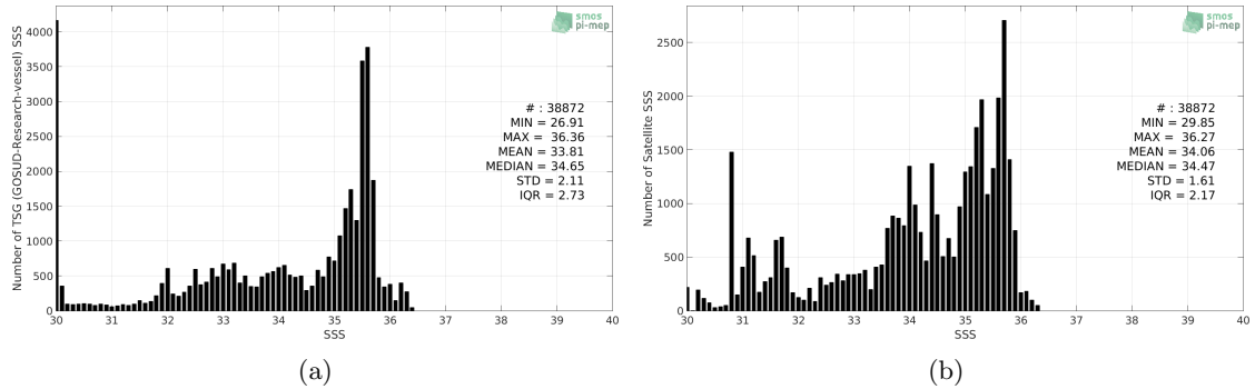
Figure 2: Histograms of SSS from TSG (GOSUD-Research-vessel) (a) and SMOS L3 v2 - 9-Days (BEC) (b) considering all match-up pairs per bins of 0.1 over the Congo river plume Pi-MEP region and for the full satellite product period.
