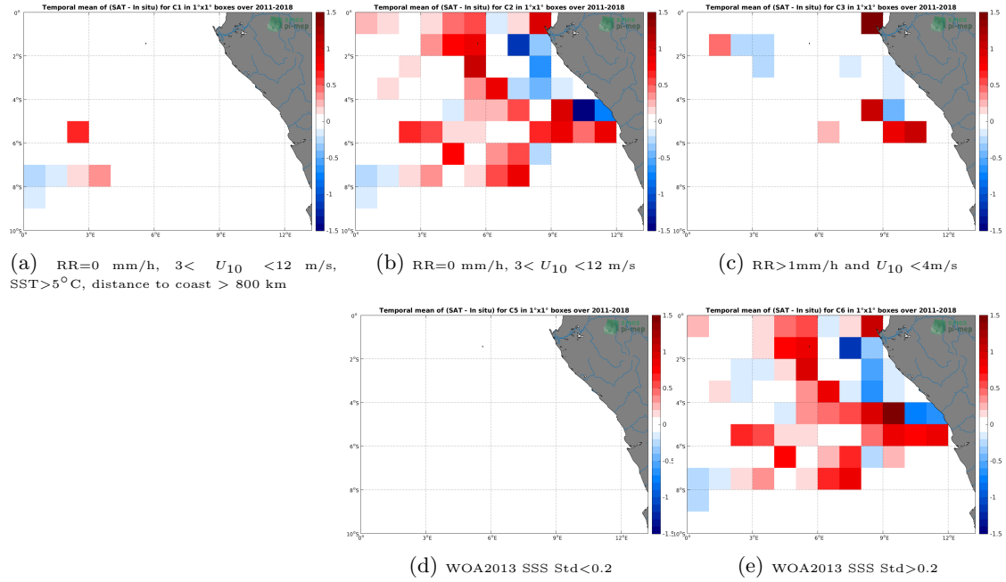
Figure 12: Temporal mean gridded over spatial boxes of size 1^\circ \times 1^\circ of \Delta SSS (SMOS L3 v2 - 9-Days (BEC) - TSG (GOSUD-Research-vessel)) for 5 different subdatasets corresponding to: RR=0 mm/h, 3 < U_{10} < 12 m/s, SST >5^\circ\text{C} , distance to coast > 800 km (a), RR=0 mm/h, 3 < U_{10} < 12 m/s (b), RR >1 mm/h and U_{10} < 4 m/s (c), WOA2013 SSS Std <0.2 (d), WOA2013 SSS Std >0.2 (e).
