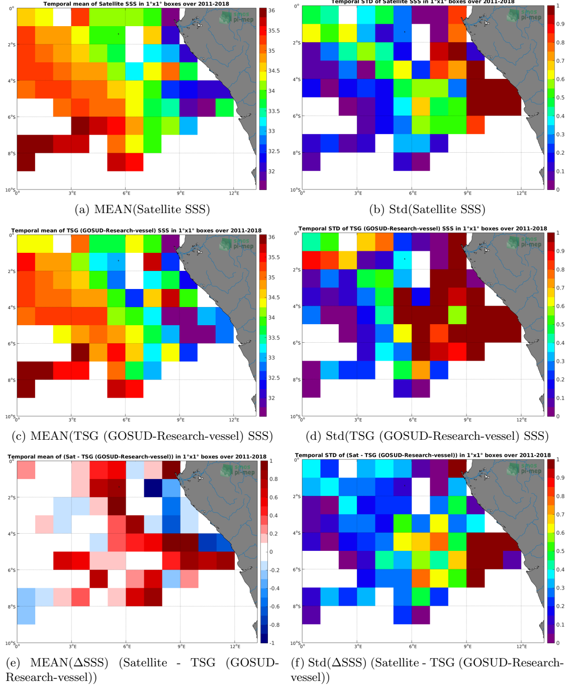
Figure 6: Temporal mean (left) and Std (right) of SSS from SMOS L3 v2 - 9-Days (BEC) (top), TSG (GOSUD-Research-vessel) (middle), and of \Delta SSS (Satellite - TSG (GOSUD-Research-vessel)). Only match-up pairs are used to generate these maps.
