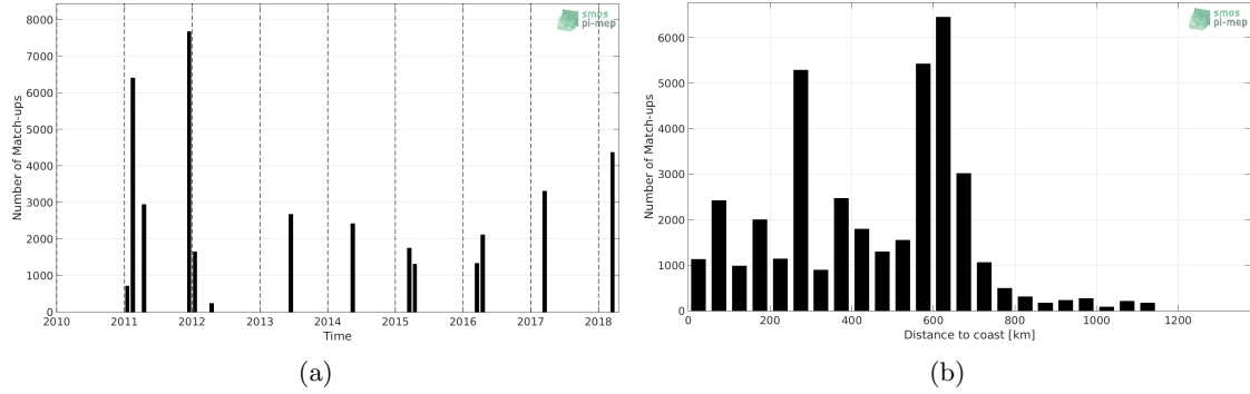
Figure 1: Number of match-ups between TSG (GOSUD-Research-vessel) and SMOS L3 v2 - 9-Days (BEC) SSS as a function of time (a) and as function of the distance to coast (b) over the Congo river plume Pi-MEP region and for the full satellite product period.
