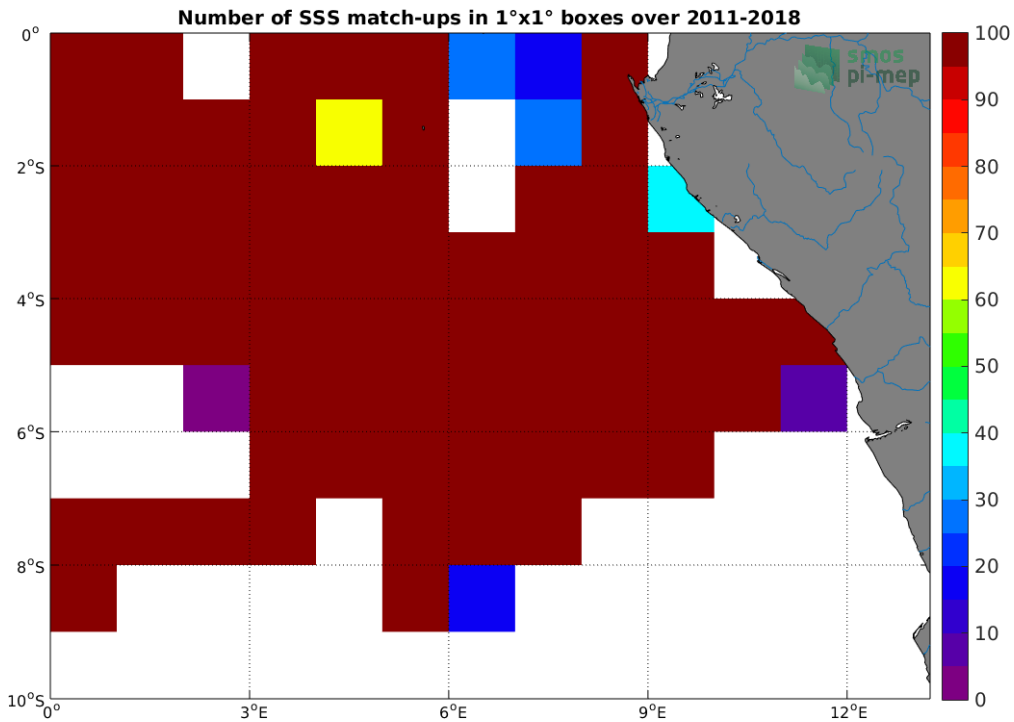
Figure 4: Number of SSS match-ups between TSG (GOSUD-Research-vessel) SSS and the SMOS L3 v2 - 9-Days (BEC) SSS product for the Congo river plume Pi-MEP region over 1^\circ \times 1^\circ boxes and for the full satellite product period.
