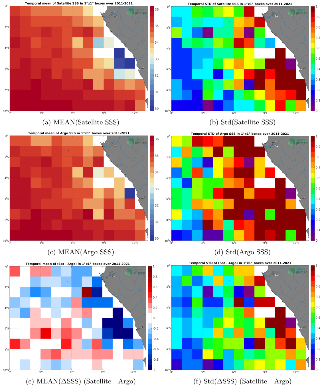
Figure 6: Temporal mean (left) and Std (right) of SSS from SMOS SSS L3 v2 - 9-Days (BEC) (top), Argo (middle), and of \Delta SSS (Satellite - Argo). Only match-up pairs are used to generate these maps.
