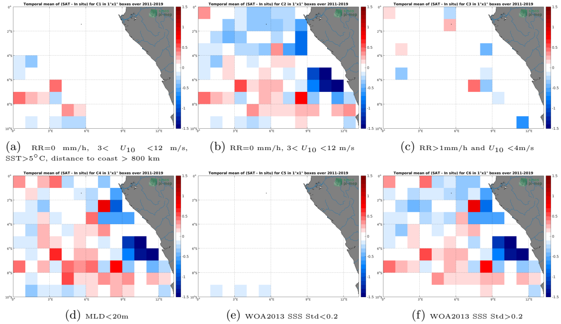
Figure 12: Temporal mean gridded over spatial boxes of size 1^\circ \times 1^\circ of \Delta SSS (SMOS SSS L3 v2 - 9-Days (BEC) - Argo) for 6 different subdatasets corresponding to: RR=0 mm/h, 3 < U_{10} < 12 m/s, SST >5^\circ\text{C} , distance to coast > 800 km (a), RR=0 mm/h, 3 < U_{10} < 12 m/s (b), RR >1 mm/h and U_{10} < 4 m/s (c),MLD <20 m (d),WOA2013 SSS Std <0.2 (e),WOA2013 SSS Std >0.2 (f).
