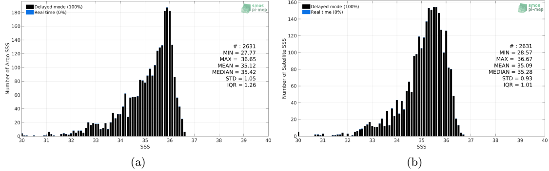
Figure 2: Histograms of SSS from Argo (a) and SMOS SSS L3 v2 - 9-Days (BEC) (b) considering all match-up pairs per bins of 0.1 over the Congo river plume Pi-MEP region and for the full satellite product period.
