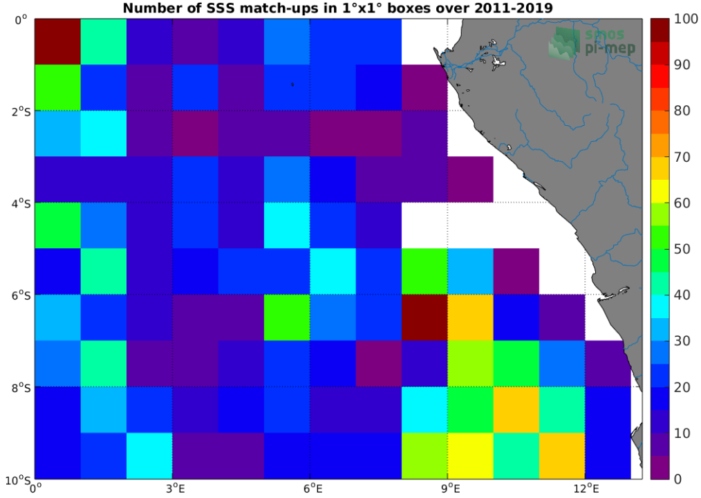
Figure 4: Number of SSS match-ups between Argo SSS and the SMOS SSS L3 v2 - 9-Days (BEC) SSS product for the Congo river plume Pi-MEP region over 1^\circ \times 1^\circ boxes and for the full satellite product period.
