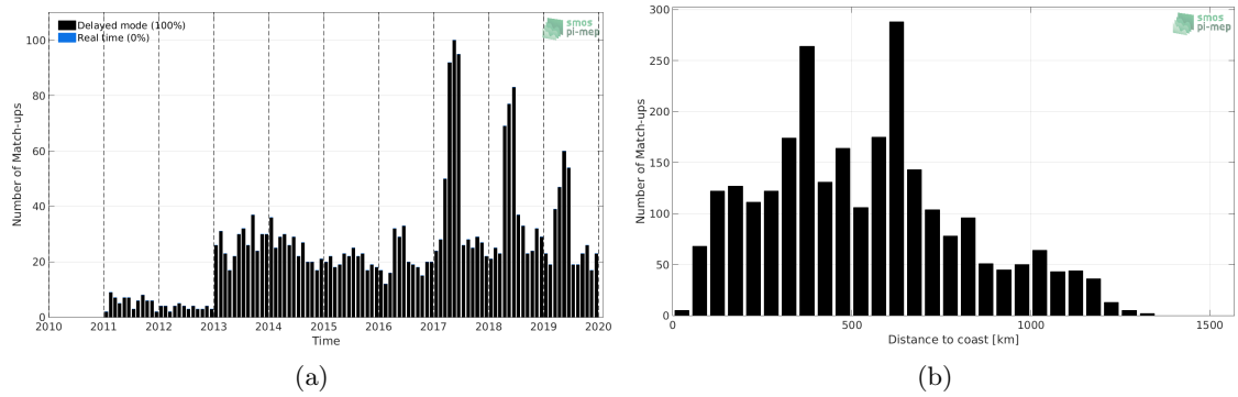
Figure 1: Number of match-ups between Argo and SMOS SSS L3 v2 - 9-Days (BEC) SSS as a function of time (a) and as function of the distance to coast (b) over the Congo river plume Pi-MEP region and for the full satellite product period.
