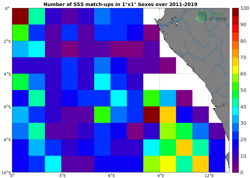
Figure 4: Number of SSS match-ups between Argo SSS and the SMOS L3 v2 - 9-Days (BEC) SSS product for the Congo river plume Pi-MEP region over 1°x1° boxes and for the full satellite product period.
