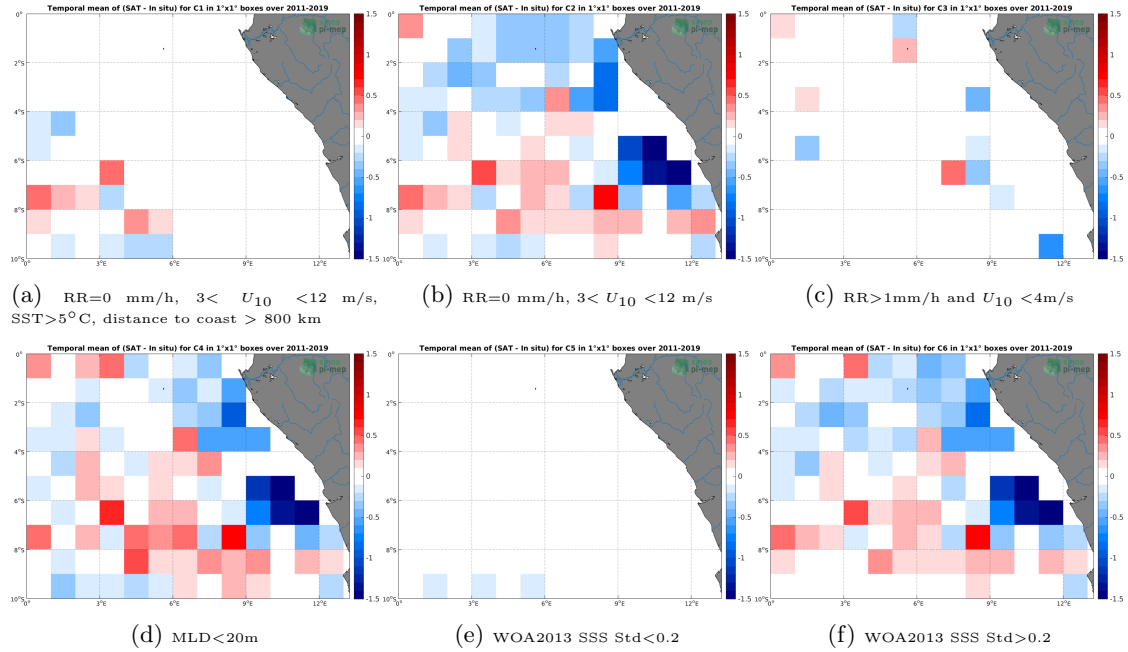
Figure 12: Temporal mean gridded over spatial boxes of size 1^\circ \times 1^\circ of \Delta SSS (SMOS L3 v2 - 9-Days (BEC) - Argo) for 6 different subdatasets corresponding to: RR=0 mm/h, 3 < U_{10} < 12 m/s, SST >5^\circ\text{C} , distance to coast > 800 km (a), RR=0 mm/h, 3 < U_{10} < 12 m/s (b), RR >1 mm/h and U_{10} < 4 m/s (c), MLD <20 m (d), WOA2013 SSS Std <0.2 (e), WOA2013 SSS Std >0.2 (f).
