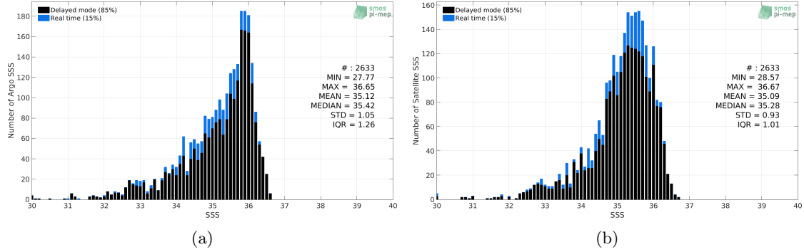
Figure 2: Histograms of SSS from Argo (a) and SMOS L3 v2 - 9-Days (BEC) (b) considering all match-up pairs per bins of 0.1 over the Congo river plume Pi-MEP region and for the full satellite product period.
