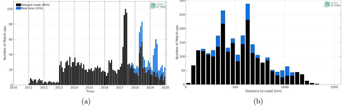
Figure 1: Number of match-ups between Argo and SMOS L3 v2 - 9-Days (BEC) SSS as a function of time (a) and as function of the distance to coast (b) over the Congo river plume Pi-MEP region and for the full satellite product period.
