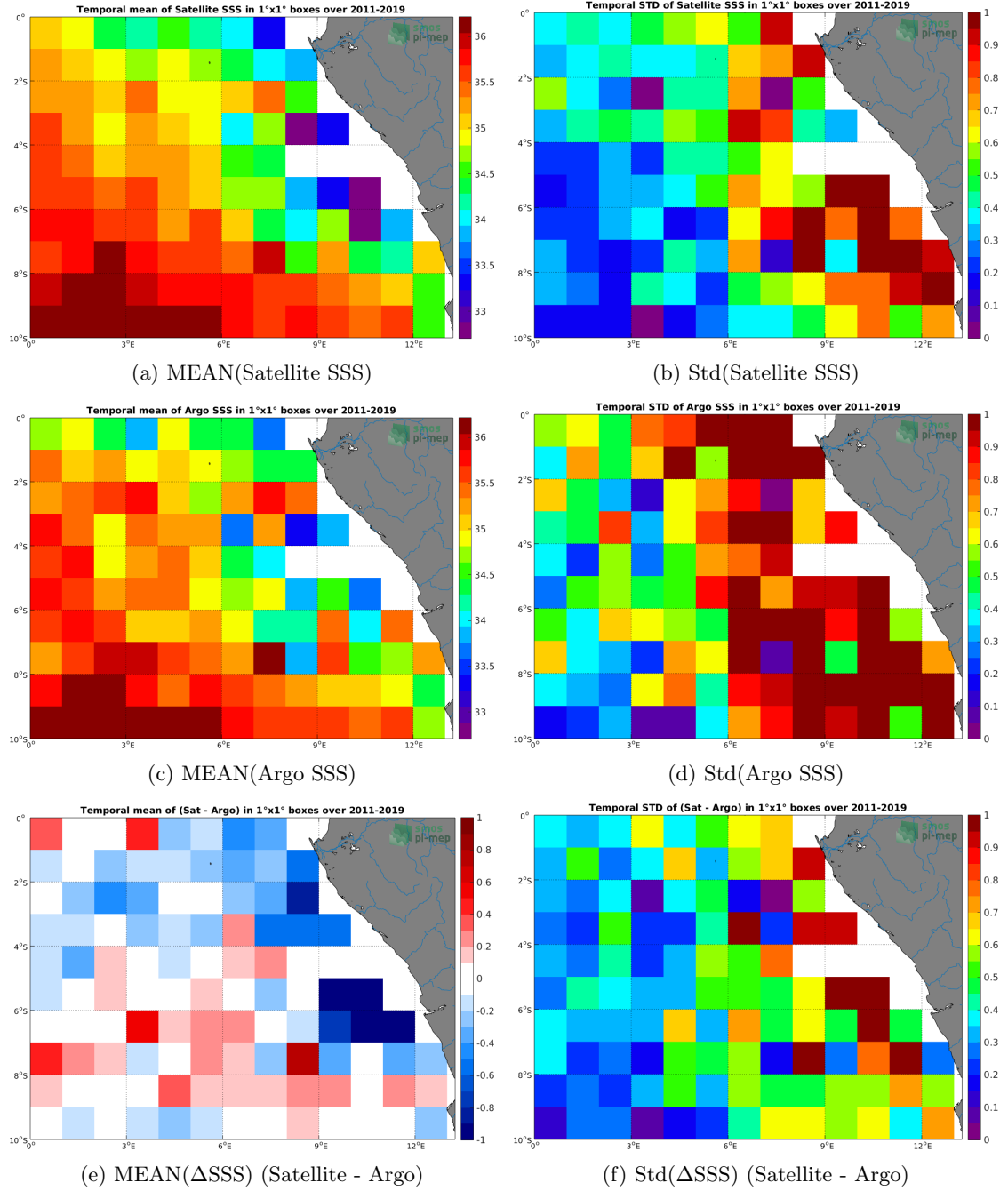
Figure 6: Temporal mean (left) and Std (right) of SSS from SMOS L3 v2 - 9-Days (BEC) (top), Argo (middle), and of \Delta SSS (Satellite - Argo). Only match-up pairs are used to generate these maps.
