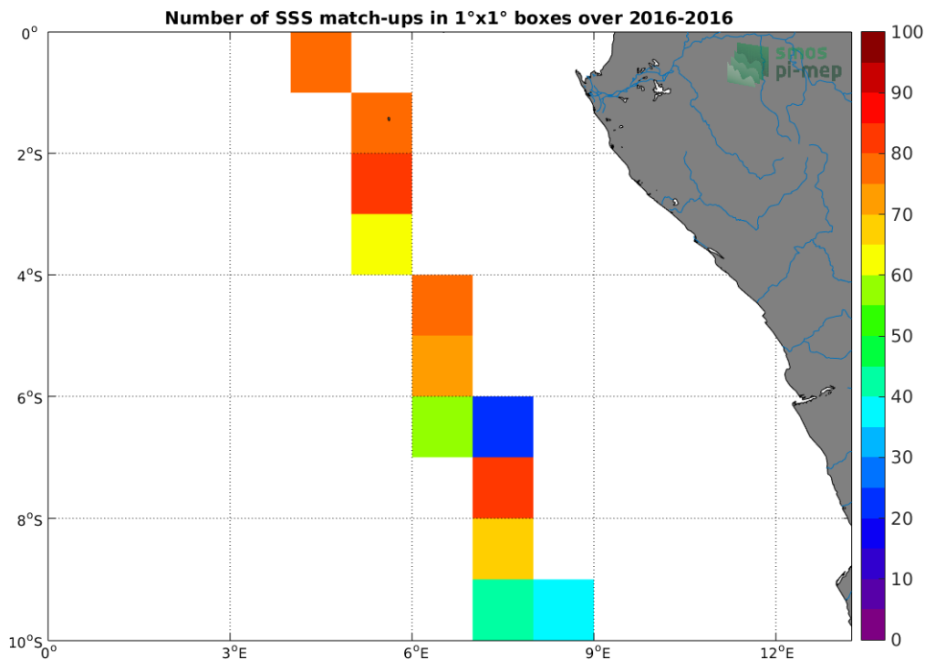
Figure 4: Number of SSS match-ups between TSG-LEGOS-DM SSS and the SMOS-L3-BEC-OA-V1-9DAYS-0.25DEG SSS product for the Congo river plume Pi-MEP region over 1°x1° boxes and for the full satellite product period.
