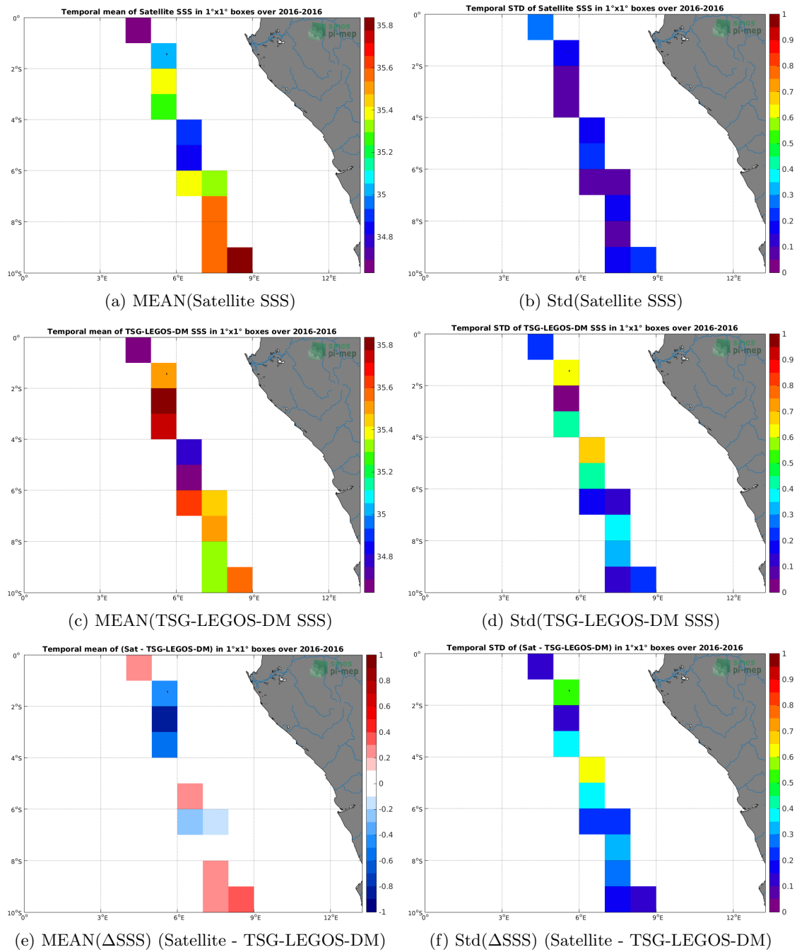
Figure 6: Temporal mean (left) and Std (right) of SSS from SMOS-L3-BEC-OA-V1-9DAYS-0.25DEG (top), TSG-LEGOS-DM (middle), and of \Delta SSS (Satellite - TSG-LEGOS-DM). Only match-up pairs are used to generate these maps.
