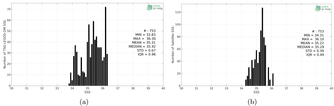
Figure 2: Histograms of SSS from TSG-LEGOS-DM (a) and SMOS-L3-BEC-OA-V1-9DAYS-0.25DEG (b) considering all match-up pairs per bins of 0.1 over the Congo river plume Pi-MEP region and for the full satellite product period.
