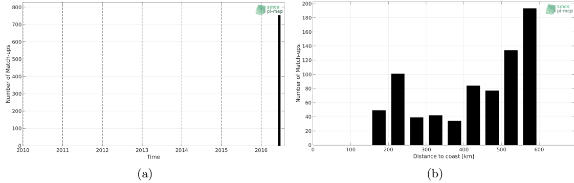
Figure 1: Number of match-ups between TSG-LEGOS-DM and SMOS-L3-BEC-OA-V1-9DAYS-0.25DEG SSS as a function of time (a) and as function of the distance to coast (b) over the Congo river plume Pi-MEP region and for the full satellite product period.
