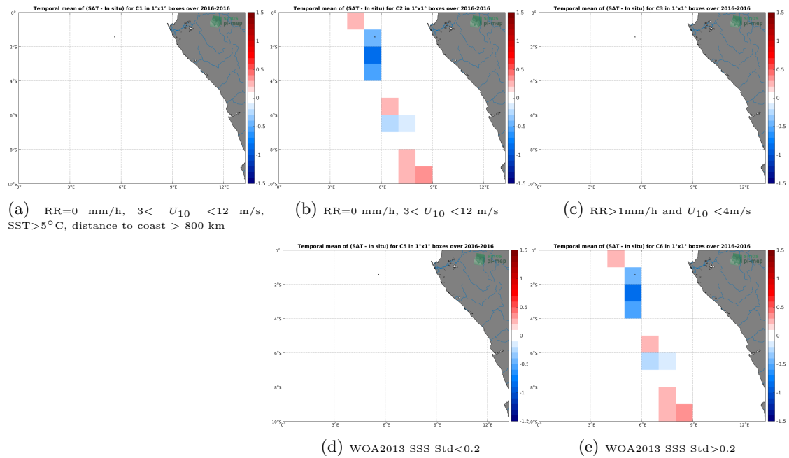
Figure 12: Temporal mean gridded over spatial boxes of size 1^\circ \times 1^\circ of \Delta SSS (SMOS-L3-BEC-OA-V1-9DAYS-0.25DEG - TSG-LEGOS-DM) for 5 different subdatasets corresponding to:RR=0 mm/h, 3 < U_{10} < 12 m/s, SST > 5^\circ\text{C} , distance to coast > 800 km (a), RR=0 mm/h, 3 < U_{10} < 12 m/s (b), RR > 1 mm/h and U_{10} < 4 m/s (c), WOA2013 SSS Std < 0.2 (d), WOA2013 SSS Std > 0.2 (e).
