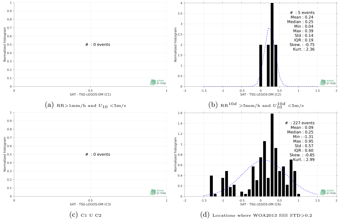
Figure 13: Normalized histogram of \Delta\text{SSS} (SMOS-L3-BEC-OA-V1-9DAYS-0.25DEG - TSG-LEGOS-DM) for 6 different subdatasets corresponding to: RR > 1\text{mm/h} and U_{10} < 5\text{m/s} (a), RR^{10d} > 5\text{mm/h} and U_{10}^{10d} < 5\text{m/s} (b), C1 \cup C2 (c), Locations where WOA2013 SSS STD > 0.2 (d).
