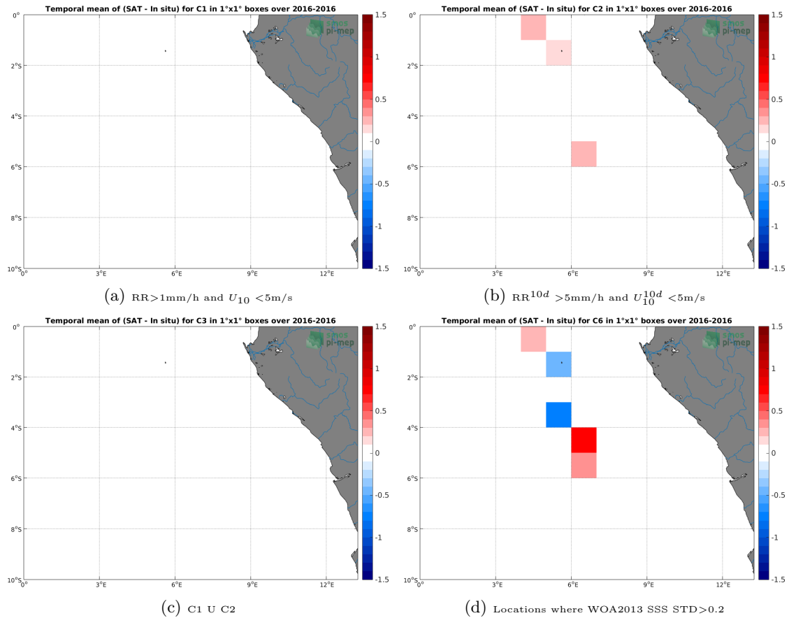
Figure 12: Temporal mean gridded over spatial boxes of size 1^\circ \times 1^\circ of \Delta SSS (SMOS-L3-BEC-OA-V1-9DAYS-0.25DEG - TSG-LEGOS-DM) for 4 different subdatasets corresponding to: RR > 1\text{mm/h} and U_{10} < 5\text{m/s} (a), RR^{10d} > 5\text{mm/h} and U_{10}^{10d} < 5\text{m/s} (b), C1 \cup C2 (c), Locations where WOA2013 SSS STD > 0.2 (d).
