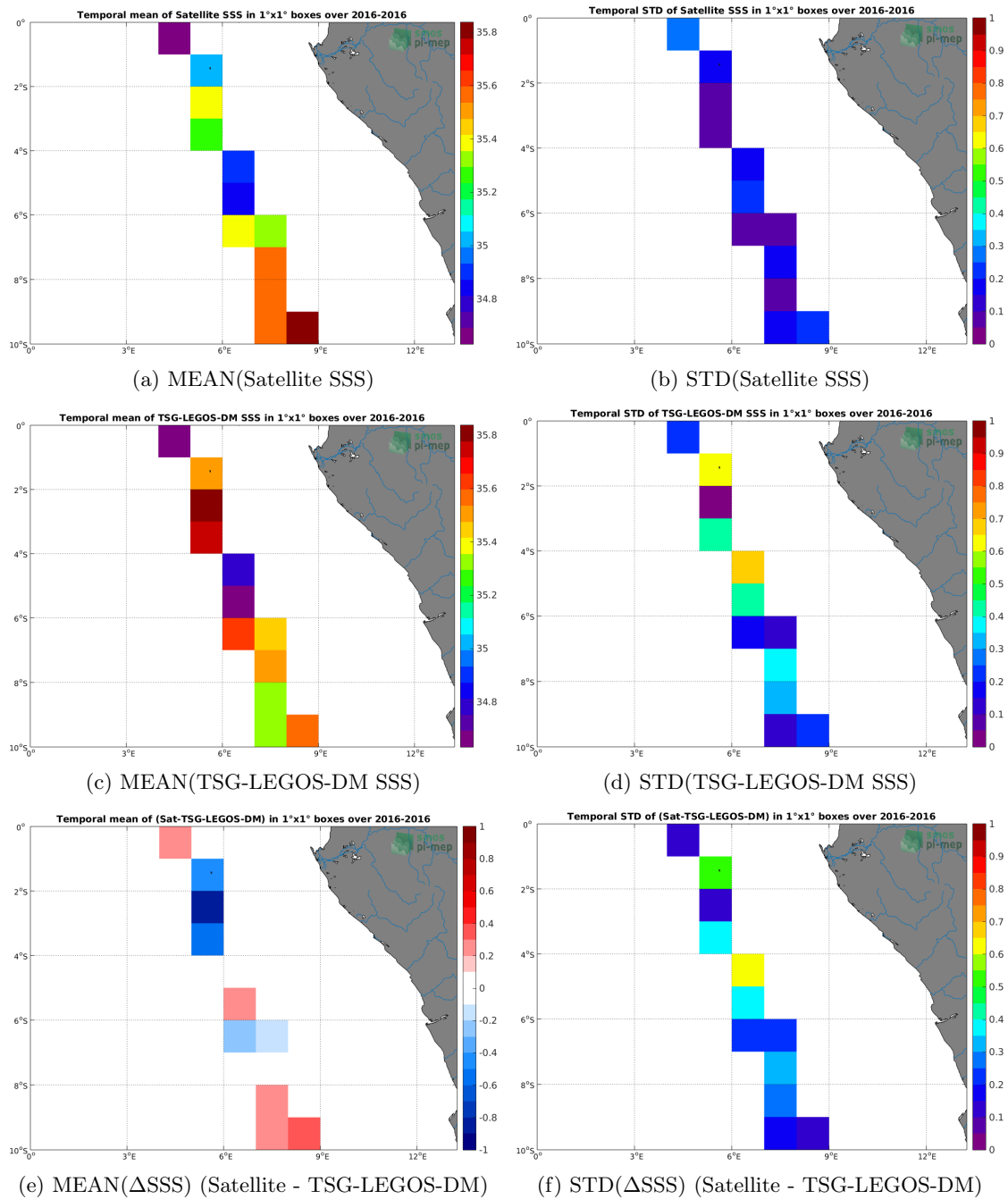
Figure 6: Temporal mean (left) and STD (right) of SSS from SMOS-L3-BEC-OA-V1-9DAYS-0.25DEG (top), TSG-LEGOS-DM (middle), and of \Delta SSS (Satellite - TSG-LEGOS-DM). Only match-up pairs are used to generate these maps.
