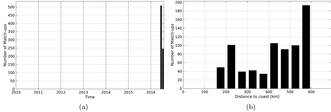
Figure 1: Number of match-ups between TSG-LEGOS-DM and SMOS-L3-BEC-OA-V1-9DAYS-0.25DEG SSS as a function of time (a) and as function of the distance to coast (b) over the Congo river plume Pi-MEP region and for the full satellite product period.
