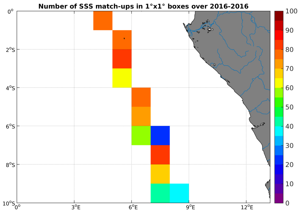
Figure 4: Number of SSS match-ups between TSG-LEGOS-DM SSS and the SMOS-L3-BEC-OA-V1-9DAYS-0.25DEG SSS product for the Congo river plume Pi-MEP region over 1^\circ \times 1^\circ boxes and for the full satellite product period.
