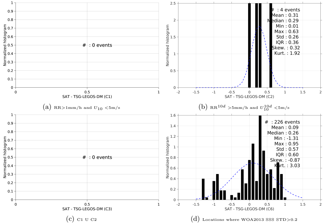
Figure 13: Normalized histogram of \Delta\text{SSS} (SMOS-L3-BEC-OA-V1-9DAYS-0.25DEG - TSG-LEGOS-DM) for 6 different subdatasets corresponding to: RR > 1\text{mm/h} and U_{10} < 5\text{m/s} (a), RR^{10d} > 5\text{mm/h} and U_{10}^{10d} < 5\text{m/s} (b), C1 U C2 (c), Locations where WOA2013 SSS STD > 0.2 (d).
