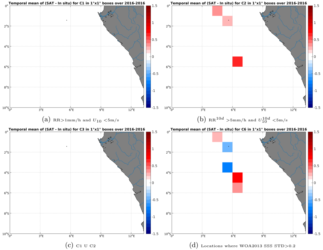
Figure 12: Temporal mean gridded over spatial boxes of size 1^\circ \times 1^\circ of \Delta SSS (SMOS-L3-BEC-OA-V1-9DAYS-0.25DEG - TSG-LEGOS-DM) for 4 different subdatasets corresponding to: RR > 1mm/h and U_{10} < 5 m/s (a), RR^{10d} > 5 mm/h and U_{10}^{10d} < 5 m/s (b), C1 U C2 (c), Locations where WOA2013 SSS STD > 0.2 (d).
