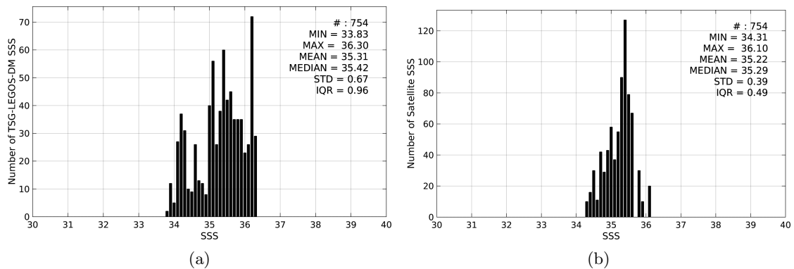
Figure 2: Histograms of SSS from TSG-LEGOS-DM (a) and SMOS-L3-BEC-OA-V1-9DAYS-0.25DEG (b) considering all match-up pairs per bins of 0.1 over the Congo river plume Pi-MEP region and for the full satellite product period.
