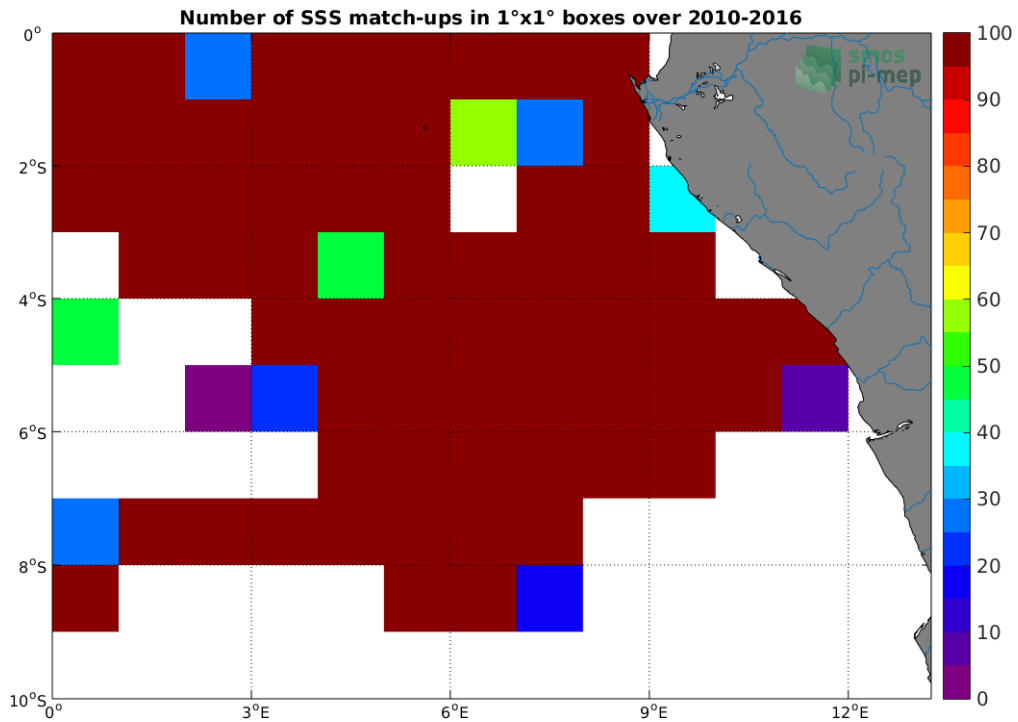
Figure 4: Number of SSS match-ups between TSG-GOSUD-Research-vessel SSS and the SMOS-L3-BEC-OA-V1-9DAYS-0.25DEG SSS product for the Congo river plume Pi-MEP region over 1°x1° boxes and for the full satellite product period.
