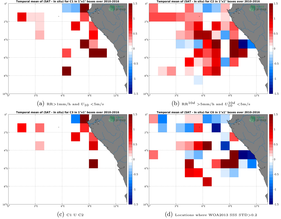
Figure 12: Temporal mean gridded over spatial boxes of size 1^\circ \times 1^\circ of \Delta SSS (SMOS-L3-BEC-OA-V1-9DAYS-0.25DEG - TSG-GOSUD-Research-vessel) for 4 different subdatasets corresponding to: RR > 1\text{mm/h} and U_{10} < 5\text{m/s} (a), RR^{10d} > 5\text{mm/h} and U_{10}^{10d} < 5\text{m/s} (b), C1 \cup C2 (c), Locations where WOA2013 SSS STD > 0.2 (d).
