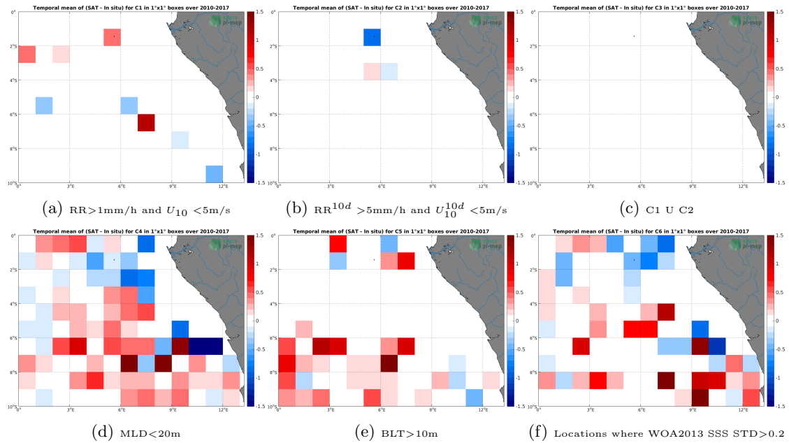
Figure 12: Temporal mean gridded over spatial boxes of size 1^\circ \times 1^\circ of \Delta\text{SSS} (SMOS-L3-BEC-OA-V1-9DAYS-0.25DEG - Argo) for 6 different subdatasets corresponding to: RR > 1\text{mm/h} and U_{10} < 5\text{m/s} (a), RR^{10d} > 5\text{mm/h} and U_{10}^{10d} < 5\text{m/s} (b), C1 U C2 (c), MLD < 20\text{m} (d), BLT > 10\text{m} (e), Locations where WOA2013 SSS STD > 0.2 (f).
