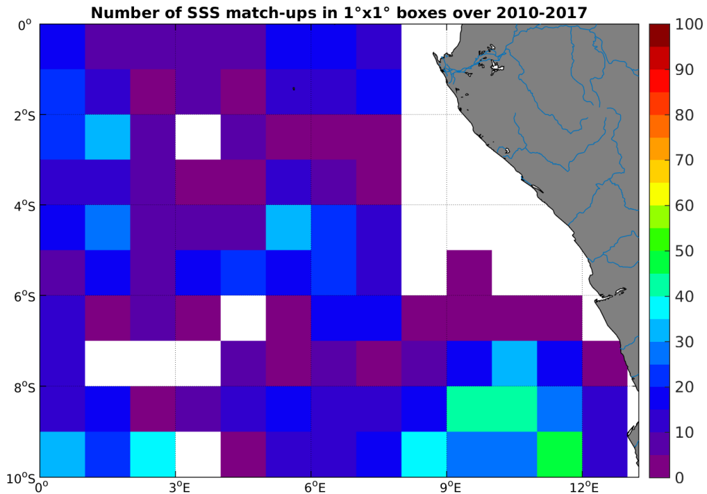
Figure 4: Number of SSS match-ups between Argo SSS and the SMOS-L3-BEC-OA-V1-9DAYS-0.25DEG SSS product for the Congo river plume Pi-MEP region over 1°x1° boxes and for the full satellite product period.
