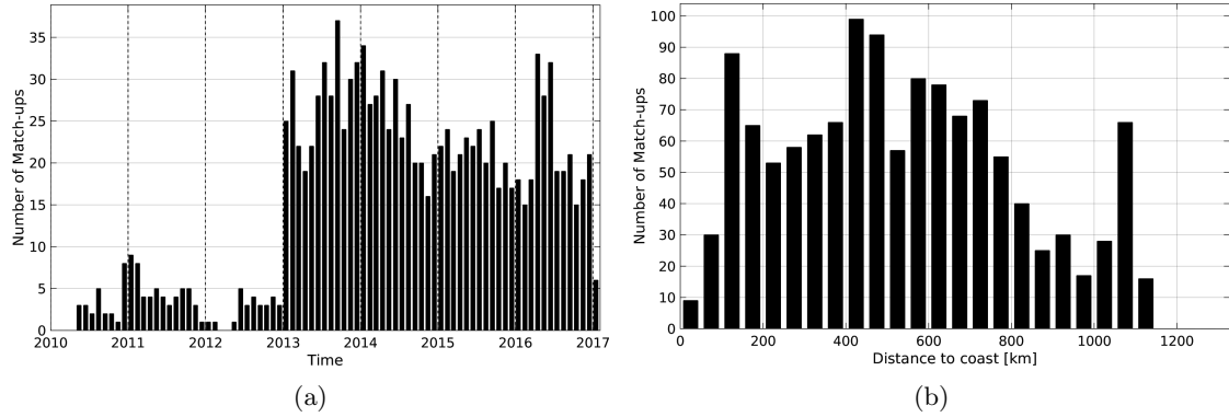
Figure 1: Number of match-ups between Argo and SMOS-L3-BEC-OA-V1-9DAYS-0.25DEG SSS as a function of time (a) and as function of the distance to coast (b) over the Congo river plume Pi-MEP region and for the full satellite product period.
