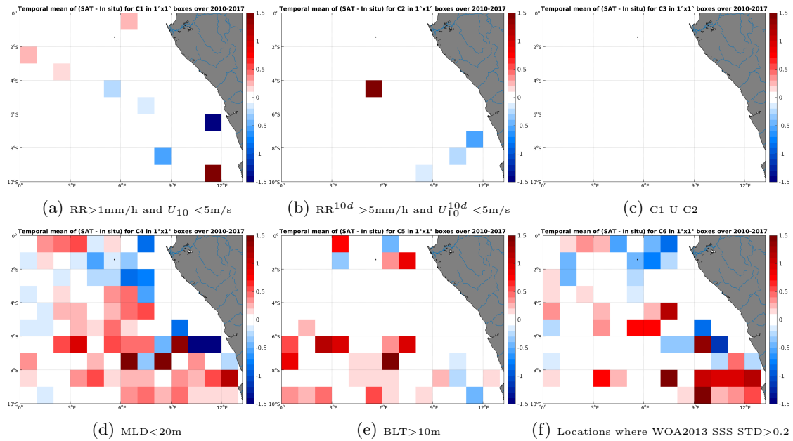
Figure 12: Temporal mean gridded over spatial boxes of size 1^\circ \times 1^\circ of \Delta SSS (SMOS-L3-BEC-OA-V1-9DAYS-0.25DEG - Argo) for 6 different subdatasets corresponding to:RR >1 mm/h and U_{10} < 5 m/s (a), RR^{10d} > 5 mm/h and U_{10}^{10d} < 5 m/s (b), C1 U C2 (c),MLD <20 m (d),BLT >10 m (e),Locations where WOA2013 SSS STD >0.2 (f).
