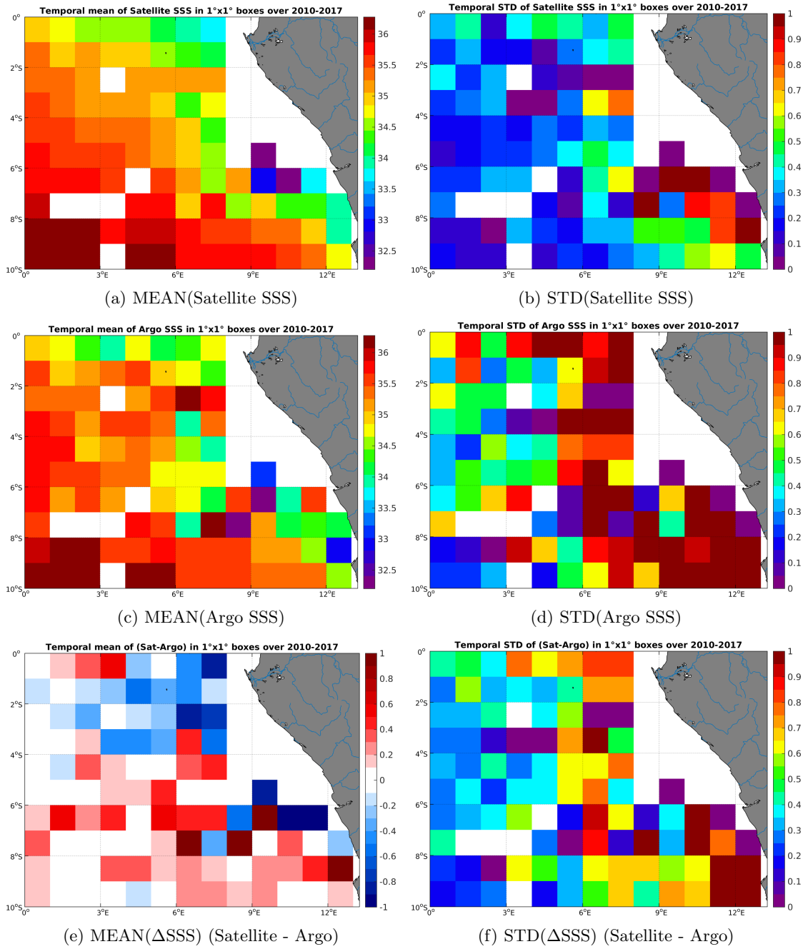
Figure 6: Temporal mean (left) and STD (right) of SSS from SMOS-L3-BEC-OA-V1-9DAYS-0.25DEG (top), Argo (middle), and of \Delta SSS (Satellite - Argo). Only match-up pairs are used to generate these maps.
