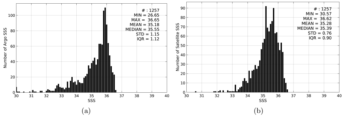
Figure 2: Histograms of SSS from Argo (a) and SMOS-L3-BEC-OA-V1-9DAYS-0.25DEG (b) considering all match-up pairs per bins of 0.1 over the Congo river plume Pi-MEP region and for the full satellite product period.
