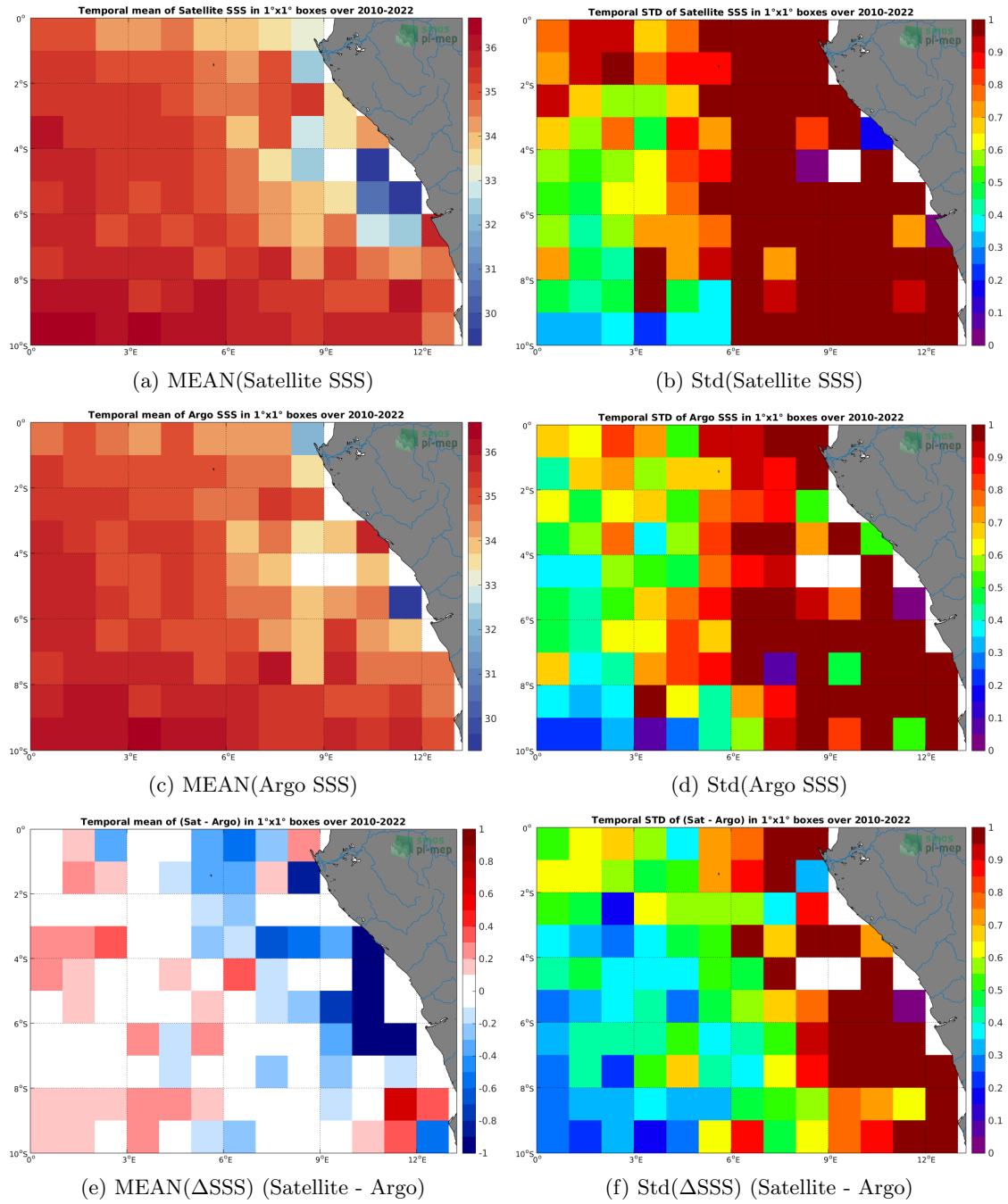
Figure 6: Temporal mean (left) and Std (right) of SSS from SMOS SSS L2-AVERAGED v700 (ESA) (top), Argo (middle), and of \Delta SSS (Satellite - Argo). Only match-up pairs are used to generate these maps.
