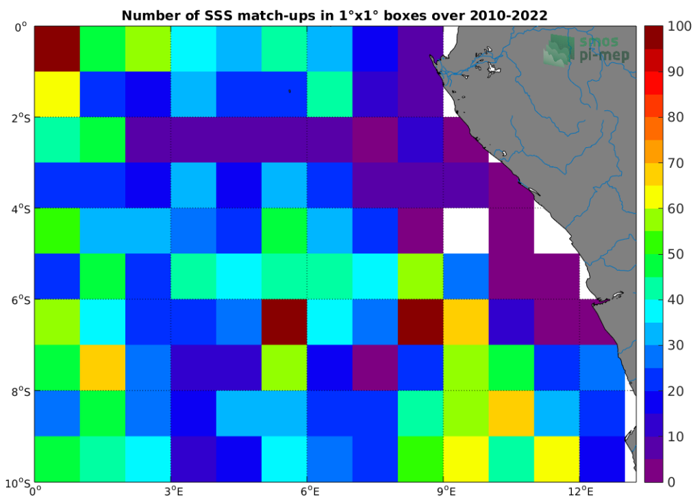
Figure 4: Number of SSS match-ups between Argo SSS and the SMOS SSS L2-AVERAGED v700 (ESA) SSS product for the Congo river plume Pi-MEP region over 1^{\circ} \times 1^{\circ} boxes and for the full satellite product period.
