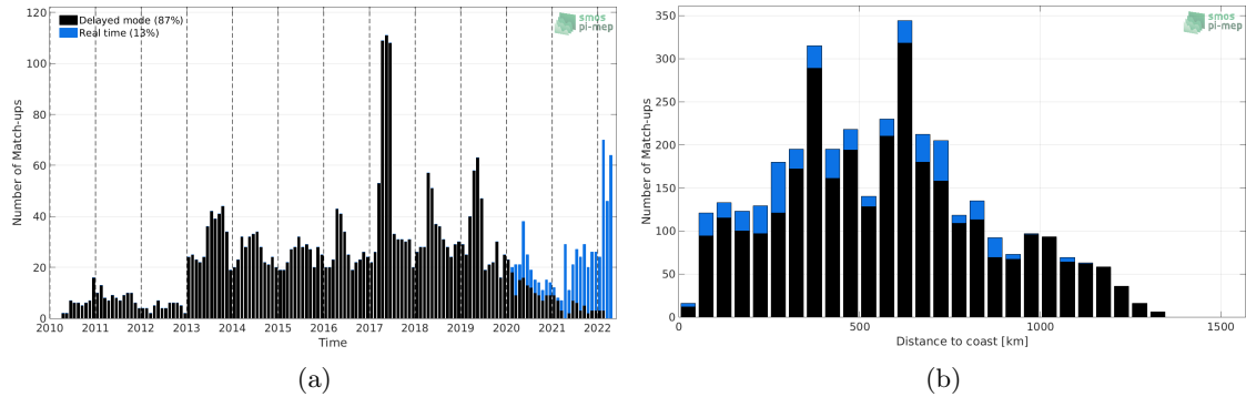
Figure 1: Number of match-ups between Argo and SMOS SSS L2-AVERAGED v700 (ESA) SSS as a function of time (a) and as function of the distance to coast (b) over the Congo river plume Pi-MEP region and for the full satellite product period.
