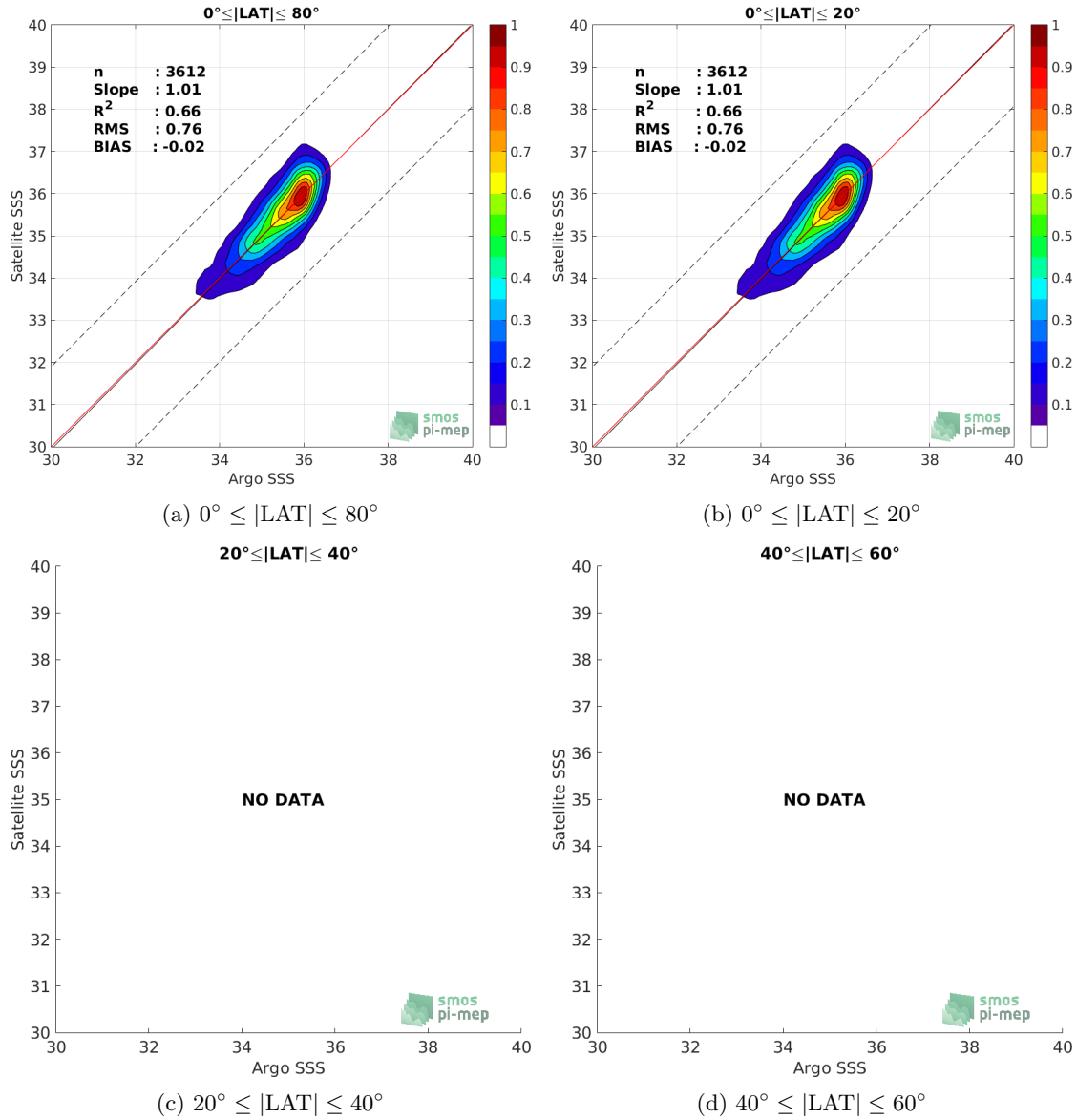
Figure 9: Contour maps of the concentration of SMOS SSS L2-AVERAGED v700 (ESA) SSS (y-axis) versus Argo SSS (x-axis) at match-up pairs for different latitude bands. For each plot, the red line shows x=y . The black thin and dashed lines indicate a linear fit through the data cloud and the \pm 95\% confidence levels, respectively. The number match-up pairs n , the slope and R^2 coefficient of the linear fit, the root mean square (RMS) and the mean bias between satellite and in situ data are indicated for each latitude band in each plots.
