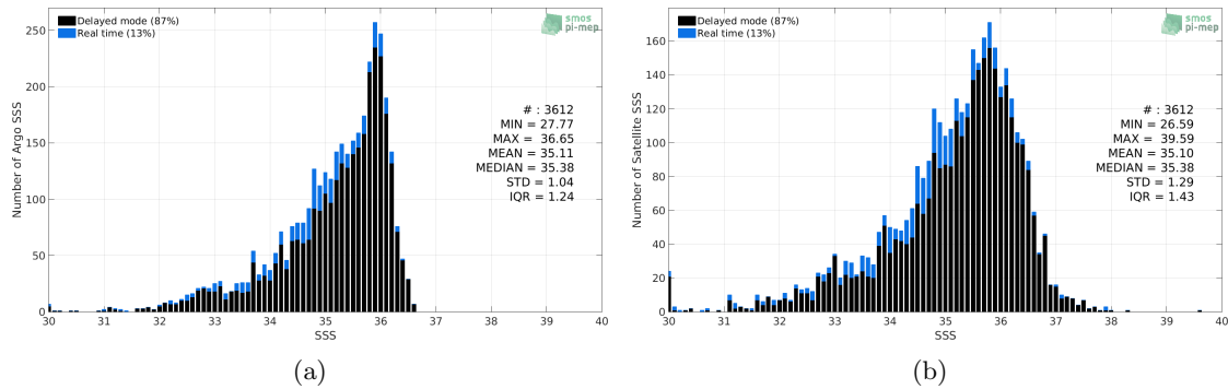
Figure 2: Histograms of SSS from Argo (a) and SMOS SSS L2-AVERAGED v700 (ESA) (b) considering all match-up pairs per bins of 0.1 over the Congo river plume Pi-MEP region and for the full satellite product period.
