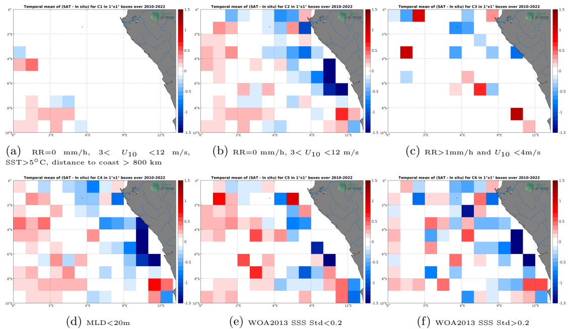
Figure 12: Temporal mean gridded over spatial boxes of size 1^\circ \times 1^\circ of \Delta SSS (SMOS SSS L2-AVERAGED v700 (ESA) - Argo) for 6 different subdatasets corresponding to:RR=0 mm/h, 3 < U_{10} < 12 m/s, SST >5^\circ C, distance to coast > 800 km (a), RR=0 mm/h, 3 < U_{10} < 12 m/s (b), RR >1 mm/h and U_{10} < 4 m/s (c),MLD <20 m (d),WOA2013 SSS Std <0.2 (e),WOA2013 SSS Std >0.2 (f).
