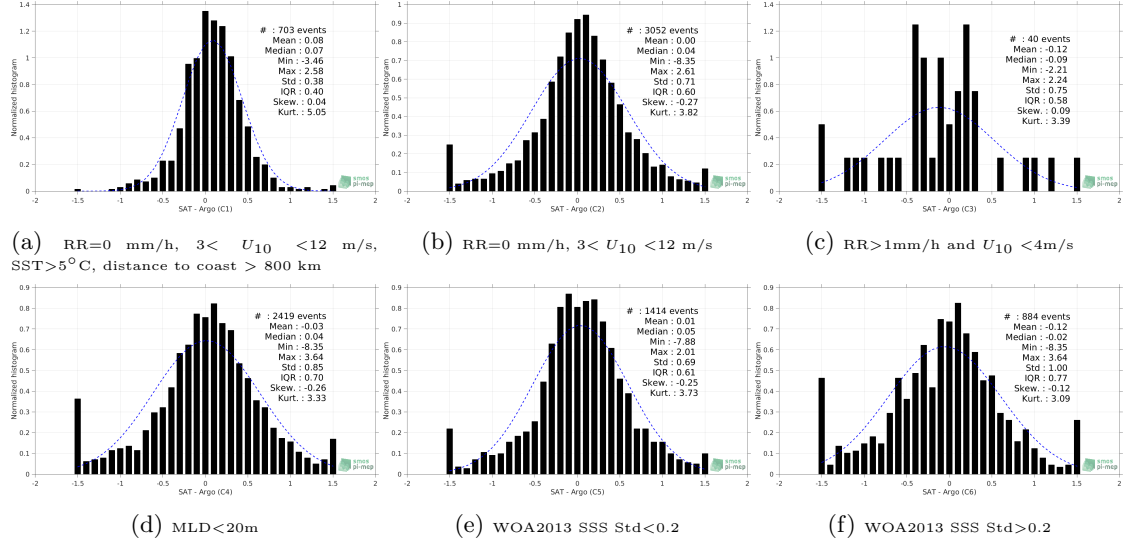
Figure 13: Normalized histogram of \Delta\text{SSS} (SMOS SSS L2-AVERAGED v700 (ESA) - Argo) for 6 different subdatasets corresponding to: RR=0 mm/h, 3 < U_{10} < 12 m/s, SST>5°C, distance to coast > 800 km (a), RR=0 mm/h, 3 < U_{10} < 12 m/s (b), RR>1mm/h and U_{10} < 4 m/s (c), MLD<20m (d), WOA2013 SSS Std<0.2 (e), WOA2013 SSS Std>0.2 (f).
