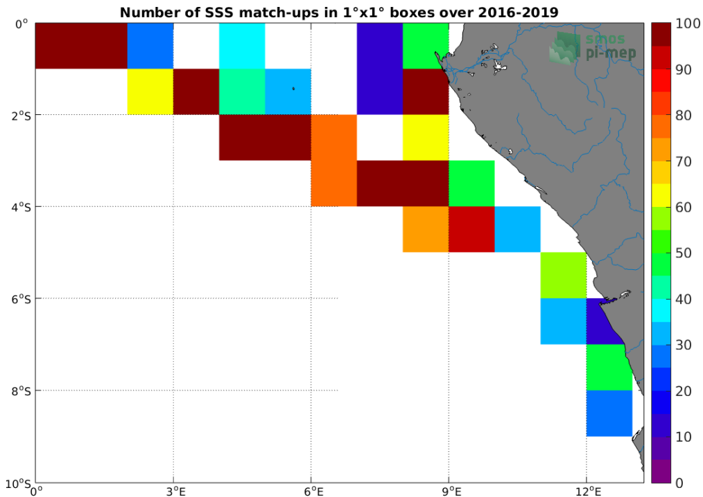
Figure 4: Number of SSS match-ups between TSG (LEGOS-DM) SSS and the SMOS SSS L2 v700 (ESA) SSS product for the Congo river plume Pi-MEP region over 1^{\circ} \times 1^{\circ} boxes and for the full satellite product period.
