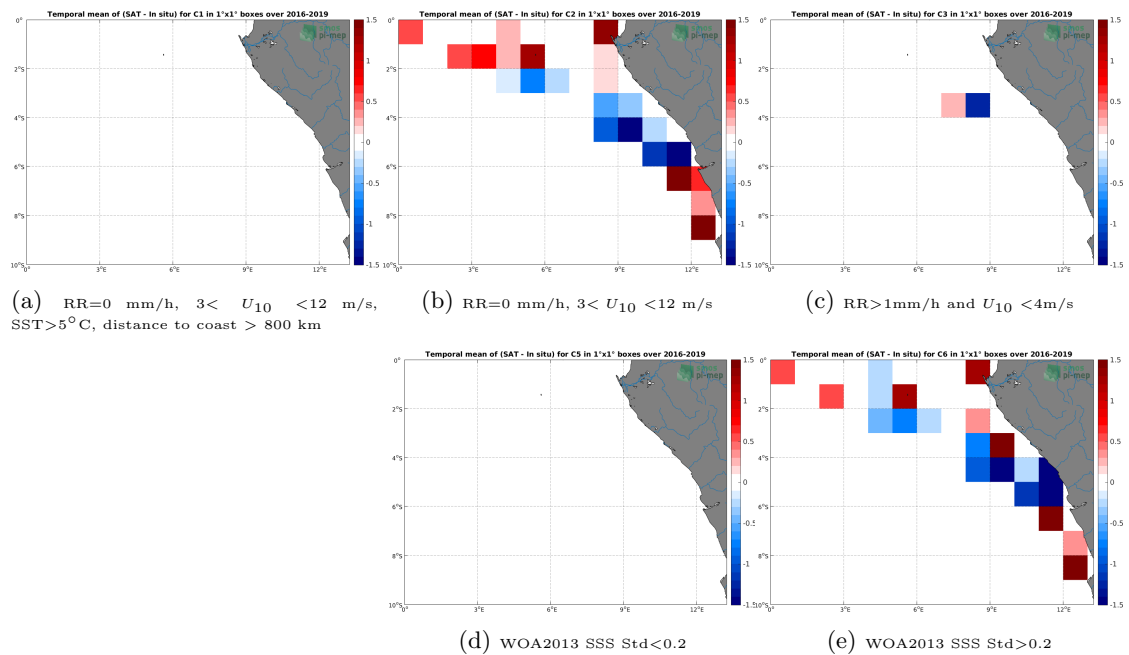
Figure 12: Temporal mean gridded over spatial boxes of size 1°x1° of \Delta SSS (SMOS SSS L2 v700 (ESA) - TSG (LEGOS-DM)) for 5 different subdatasets corresponding to:RR=0 mm/h, 3 < U_{10} < 12 m/s, SST>5°C, distance to coast > 800 km (a), RR=0 mm/h, 3 < U_{10} < 12 m/s (b), RR>1mm/h and U_{10} < 4 m/s (c), WOA2013 SSS Std<0.2 (d), WOA2013 SSS Std>0.2 (e).
