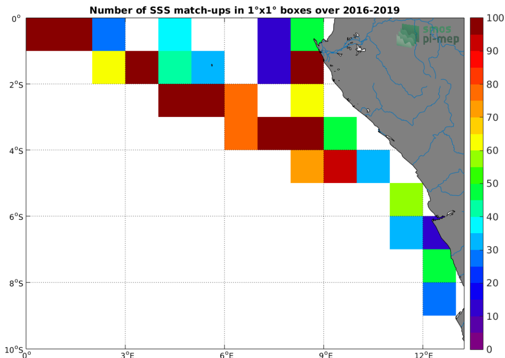
Figure 4: Number of SSS match-ups between TSG (LEGOS-DM) SSS and the SMOS SSS L2 v700 (ESA) SSS product for the Congo river plume Pi-MEP region over 1°x1° boxes and for the full satellite product period.
