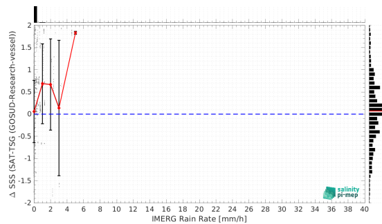
(f) IMERG Rain rate
