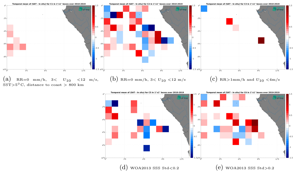
Figure 14: Temporal mean gridded over spatial boxes of size 1^\circ \times 1^\circ of \Delta SSS (SMOS SSS L2 v700 (ESA) - TSG (GOSUD-Research-vessel)) for 5 different subdatasets corresponding to:RR=0 mm/h, 3 < U_{10} < 12 m/s, SST>5°C, distance to coast > 800 km (a), RR=0 mm/h, 3 < U_{10} < 12 m/s (b), RR>1mm/h and U_{10} < 4 m/s (c), WOA2013 SSS Std<0.2 (d), WOA2013 SSS Std>0.2 (e).
