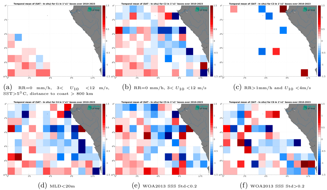
Figure 12: Temporal mean gridded over spatial boxes of size 1^\circ \times 1^\circ of \Delta SSS (SMOS SSS L2 v700 (ESA) - Argo) for 6 different subdatasets corresponding to:RR=0 mm/h, 3 < U_{10} < 12 m/s, SST >5^\circ C, distance to coast > 800 km (a), RR=0 mm/h, 3 < U_{10} < 12 m/s (b), RR >1 mm/h and U_{10} < 4 m/s (c),MLD <20 m (d),WOA2013 SSS Std <0.2 (e),WOA2013 SSS Std >0.2 (f).
