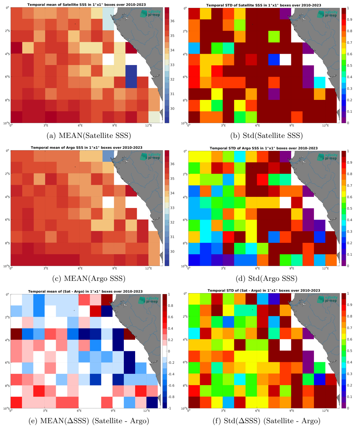
Figure 6: Temporal mean (left) and Std (right) of SSS from SMOS SSS L2 v700 (ESA) (top), Argo (middle), and of \Delta SSS (Satellite - Argo). Only match-up pairs are used to generate these maps.
