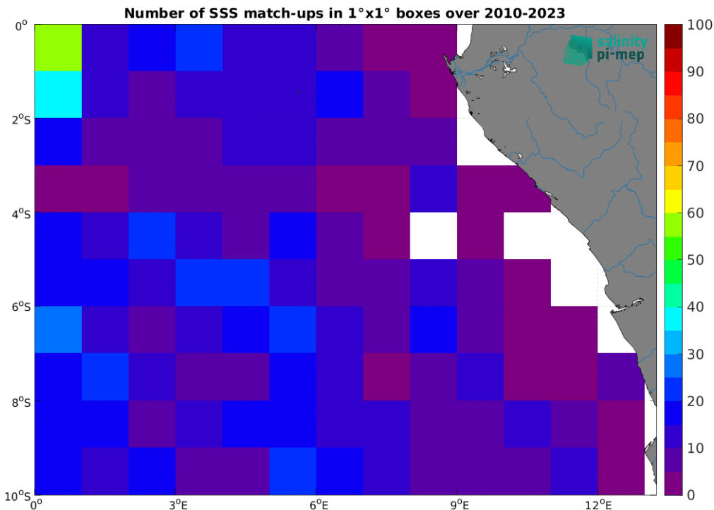
Figure 4: Number of SSS match-ups between Argo SSS and the SMOS SSS L2 v700 (ESA) SSS product for the Congo river plume Pi-MEP region over 1^{\circ} \times 1^{\circ} boxes and for the full satellite product period.
