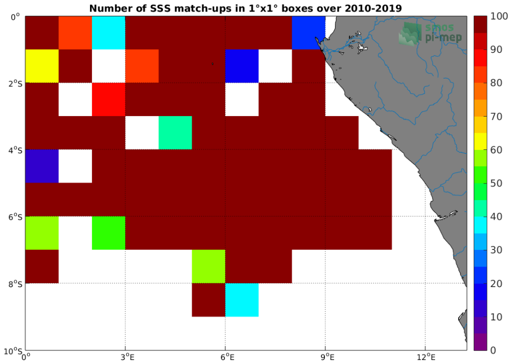
Figure 4: Number of SSS match-ups between TSG (GOSUD-Research-vessel) SSS and the SMOS SSS L2 v662 (ESA) SSS product for the Congo river plume Pi-MEP region over 1°x1° boxes and for the full satellite product period.
