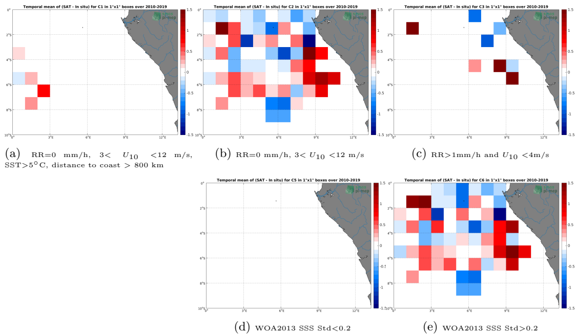
Figure 12: Temporal mean gridded over spatial boxes of size 1^\circ \times 1^\circ of \Delta SSS (SMOS SSS L2 v662 (ESA) - TSG (GOSUD-Research-vessel)) for 5 different subdatasets corresponding to:RR=0 mm/h, 3 < U_{10} < 12 m/s, SST>5°C, distance to coast > 800 km (a), RR=0 mm/h, 3 < U_{10} < 12 m/s (b), RR>1mm/h and U_{10} < 4 m/s (c), WOA2013 SSS Std<0.2 (d), WOA2013 SSS Std>0.2 (e).
