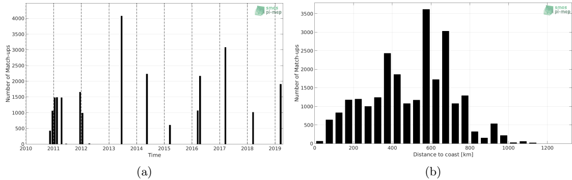
Figure 1: Number of match-ups between TSG (GOSUD-Research-vessel) and SMOS SSS L2 v662 (ESA) SSS as a function of time (a) and as function of the distance to coast (b) over the Congo river plume Pi-MEP region and for the full satellite product period.
