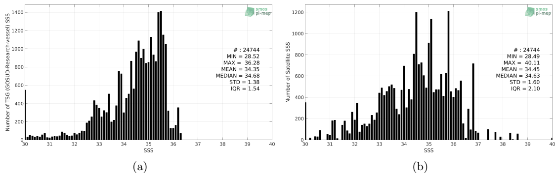
Figure 2: Histograms of SSS from TSG (GOSUD-Research-vessel) (a) and SMOS SSS L2 v662 (ESA) (b) considering all match-up pairs per bins of 0.1 over the Congo river plume Pi-MEP region and for the full satellite product period.
