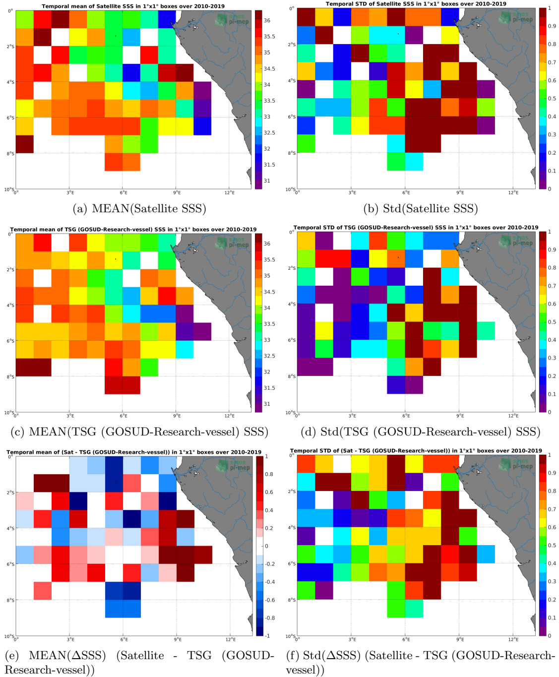
Figure 6: Temporal mean (left) and Std (right) of SSS from SMOS SSS L2 v662 (ESA) (top), TSG (GOSUD-Research-vessel) (middle), and of \Delta SSS (Satellite - TSG (GOSUD-Research-vessel)). Only match-up pairs are used to generate these maps.
