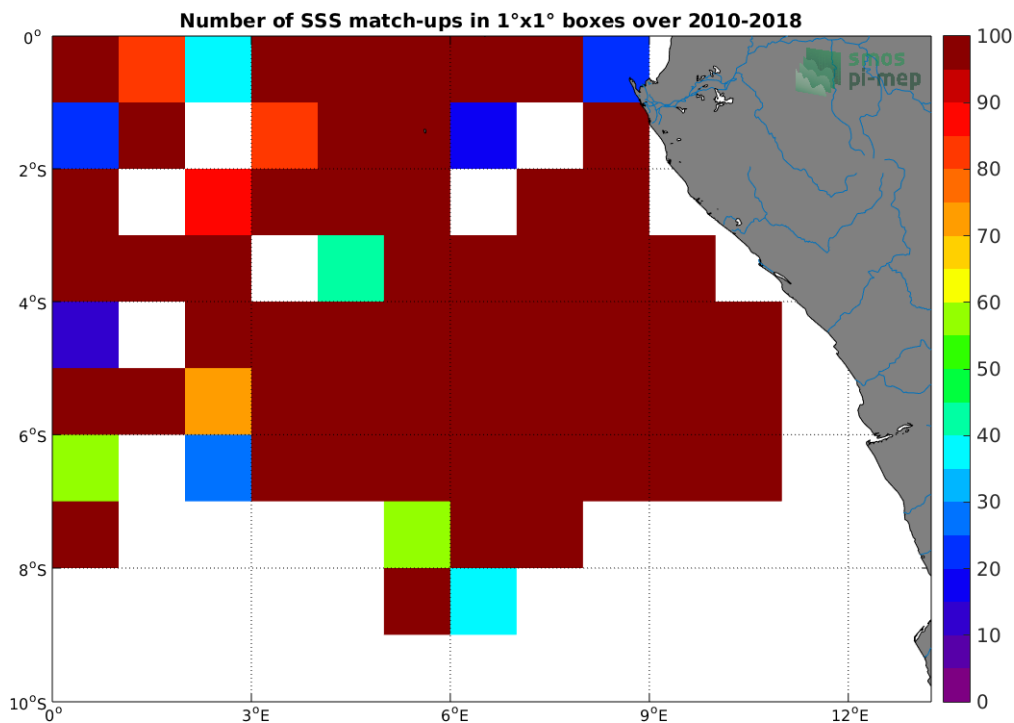
Figure 4: Number of SSS match-ups between TSG-GOSUD-Research-vessel SSS and the SMOS L2 v662 (ESA) SSS product for the Congo river plume Pi-MEP region over 1°x1° boxes and for the full satellite product period.
