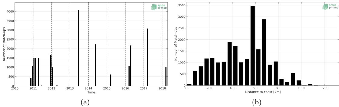
Figure 1: Number of match-ups between TSG-GOSUD-Research-vessel and SMOS L2 v662 (ESA) SSS as a function of time (a) and as function of the distance to coast (b) over the Congo river plume Pi-MEP region and for the full satellite product period.
