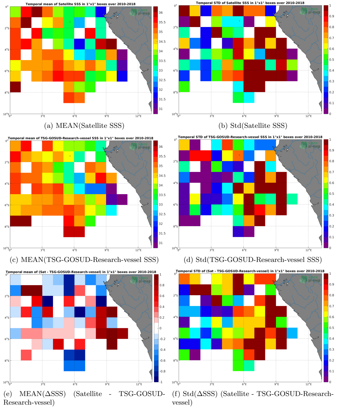
Figure 6: Temporal mean (left) and Std (right) of SSS from SMOS L2 v662 (ESA) (top), TSG-GOSUD-Research-vessel (middle), and of \Delta SSS (Satellite - TSG-GOSUD-Research-vessel). Only match-up pairs are used to generate these maps.
