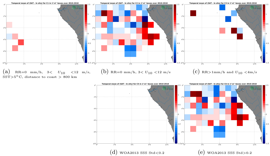
Figure 12: Temporal mean gridded over spatial boxes of size 1^\circ \times 1^\circ of \Delta SSS (SMOS L2 v662 (ESA) - TSG-GOSUD-Research-vessel) for 5 different subdatasets corresponding to:RR=0 mm/h, 3 < U_{10} < 12 m/s, SST > 5^\circ\text{C} , distance to coast > 800 km (a), RR=0 mm/h, 3 < U_{10} < 12 m/s (b), RR > 1 mm/h and U_{10} < 4 m/s (c), WOA2013 SSS Std < 0.2 (d), WOA2013 SSS Std > 0.2 (e).
