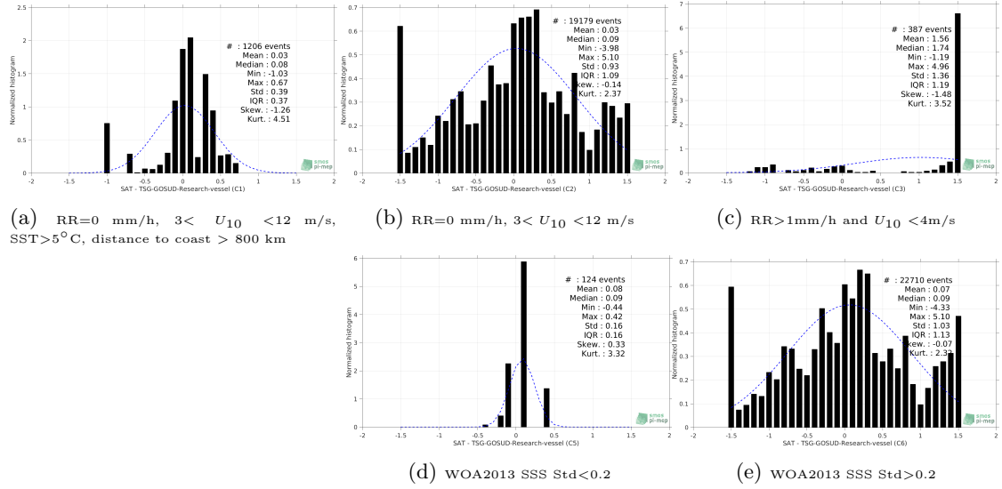
Figure 13: Normalized histogram of \Delta SSS (SMOS L2 v662 (ESA) - TSG-GOSUD-Research-vessel) for 5 different subdatasets corresponding to: RR=0 mm/h, 3 < U_{10} < 12 m/s, SST>5°C, distance to coast > 800 km (a), RR=0 mm/h, 3 < U_{10} < 12 m/s (b), RR>1mm/h and U_{10} < 4 m/s (c), WOA2013 SSS Std<0.2 (d), WOA2013 SSS Std>0.2 (e).
