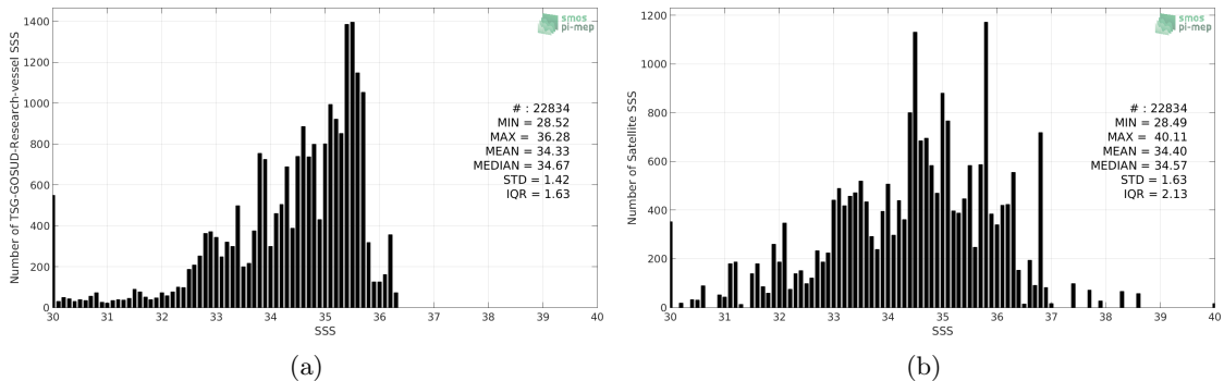
Figure 2: Histograms of SSS from TSG-GOSUD-Research-vessel (a) and SMOS L2 v662 (ESA) (b) considering all match-up pairs per bins of 0.1 over the Congo river plume Pi-MEP region and for the full satellite product period.
