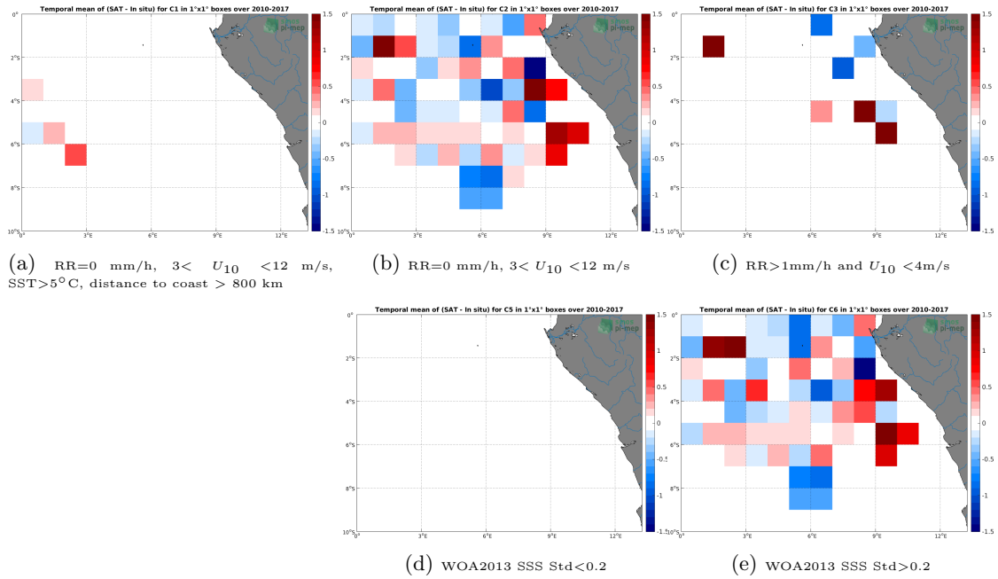
Figure 12: Temporal mean gridded over spatial boxes of size 1^\circ \times 1^\circ of \Delta SSS (SMOS-L2-DPGS-v662 - TSG-GOSUD-Research-vessel) for 5 different subdatasets corresponding to:RR=0 mm/h, 3 < U_{10} < 12 m/s, SST >5^\circ C, distance to coast > 800 km (a), RR=0 mm/h, 3 < U_{10} < 12 m/s (b), RR >1 mm/h and U_{10} < 4 m/s (c), WOA2013 SSS Std <0.2 (d), WOA2013 SSS Std >0.2 (e).
