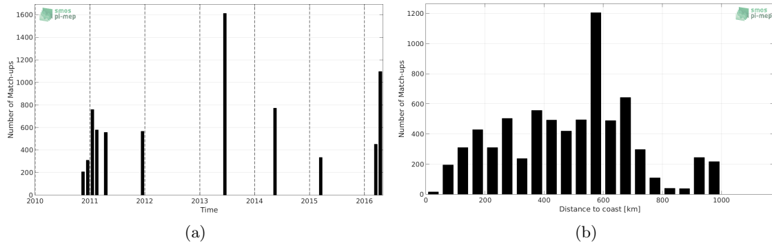
Figure 1: Number of match-ups between TSG-GOSUD-Research-vessel and SMOS-L2-DPGS-v662 SSS as a function of time (a) and as function of the distance to coast (b) over the Congo river plume Pi-MEP region and for the full satellite product period.
