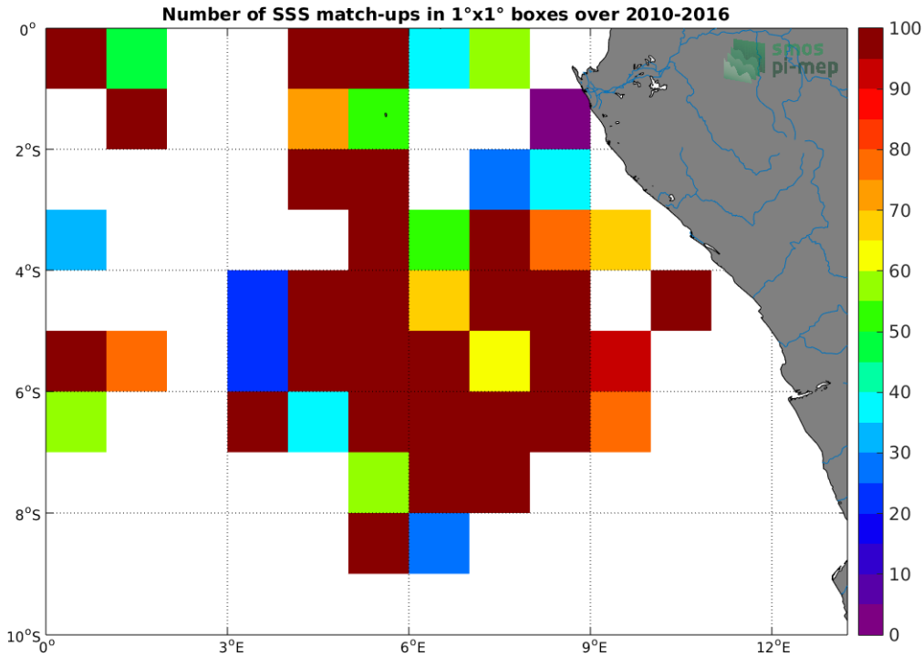
Figure 4: Number of SSS match-ups between TSG-GOSUD-Research-vessel SSS and the SMOS-L2-DPGS-v662 SSS product for the Congo river plume Pi-MEP region over 1^{\circ} \times 1^{\circ} boxes and for the full satellite product period.
