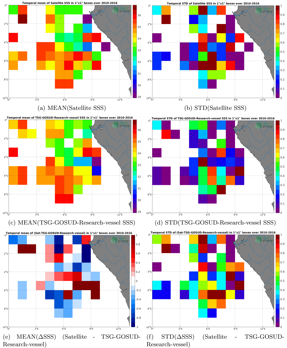
Figure 6: Temporal mean (left) and STD (right) of SSS from SMOS-L2-DPGS-v662 (top), TSG-GOSUD-Research-vessel (middle), and of \Delta SSS (Satellite - TSG-GOSUD-Research-vessel). Only match-up pairs are used to generate these maps.
