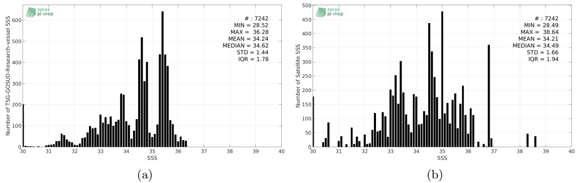
Figure 2: Histograms of SSS from TSG-GOSUD-Research-vessel (a) and SMOS-L2-DPGS-v662 (b) considering all match-up pairs per bins of 0.1 over the Congo river plume Pi-MEP region and for the full satellite product period.
