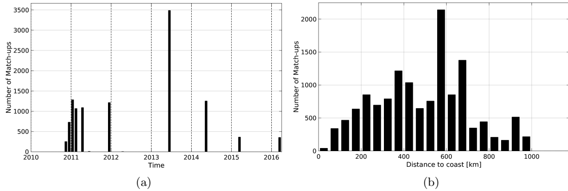
Figure 1: Number of match-ups between TSG-GOSUD-Research-vessel and SMOS-L2-DPGS-v662 SSS as a function of time (a) and as function of the distance to coast (b) over the Congo river plume Pi-MEP region and for the full satellite product period.
