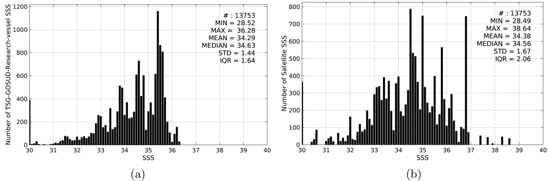
Figure 2: Histograms of SSS from TSG-GOSUD-Research-vessel (a) and SMOS-L2-DPGS-v662 (b) considering all match-up pairs per bins of 0.1 over the Congo river plume Pi-MEP region and for the full satellite product period.
