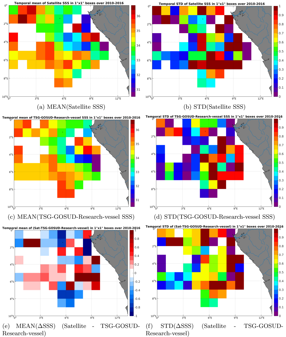
Figure 6: Temporal mean (left) and STD (right) of SSS from SMOS-L2-DPGS-v662 (top), TSG-GOSUD-Research-vessel (middle), and of \Delta SSS (Satellite - TSG-GOSUD-Research-vessel). Only match-up pairs are used to generate these maps.
