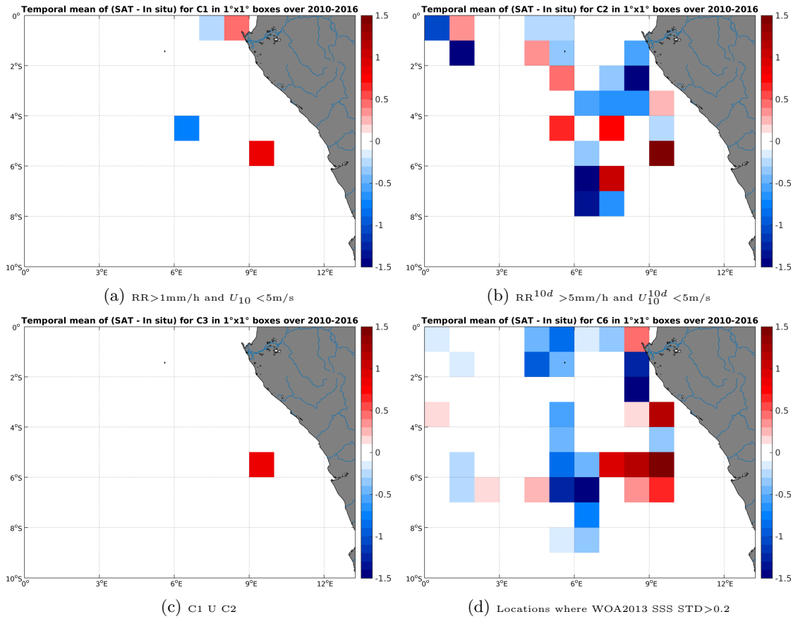
Figure 12: Temporal mean gridded over spatial boxes of size 1^\circ \times 1^\circ of \Delta SSS (SMOS-L2-DPGS-v662 - TSG-GOSUD-Research-vessel) for 4 different subdatasets corresponding to: RR > 1\text{mm/h} and U_{10} < 5\text{m/s} (a), RR^{10d} > 5\text{mm/h} and U_{10}^{10d} < 5\text{m/s} (b), C1 U C2 (c), Locations where WOA2013 SSS STD > 0.2 (d).
