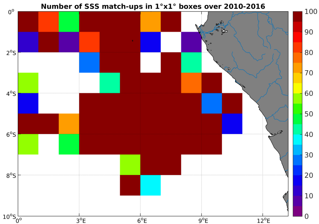
Figure 4: Number of SSS match-ups between TSG-GOSUD-Research-vessel SSS and the SMOS-L2-DPGS-v662 SSS product for the Congo river plume Pi-MEP region over 1^\circ \times 1^\circ boxes and for the full satellite product period.
