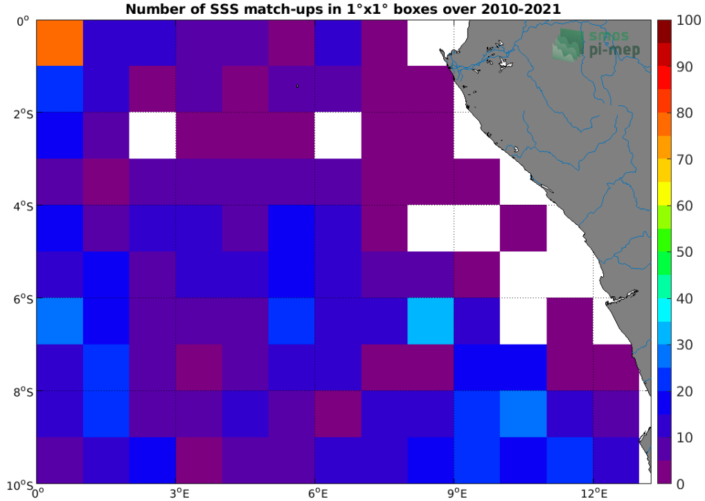
Figure 4: Number of SSS match-ups between Argo SSS and the SMOS SSS L2 v662 (ESA) SSS product for the Congo river plume Pi-MEP region over 1^\circ \times 1^\circ boxes and for the full satellite product period.
