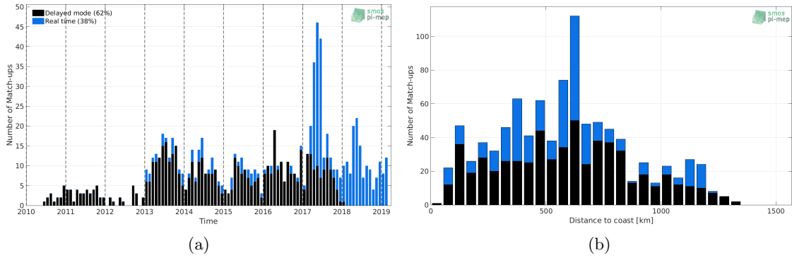
Figure 1: Number of match-ups between Argo and SMOS-L2-DPGS-v662 SSS as a function of time (a) and as function of the distance to coast (b) over the Congo river plume Pi-MEP region and for the full satellite product period.
