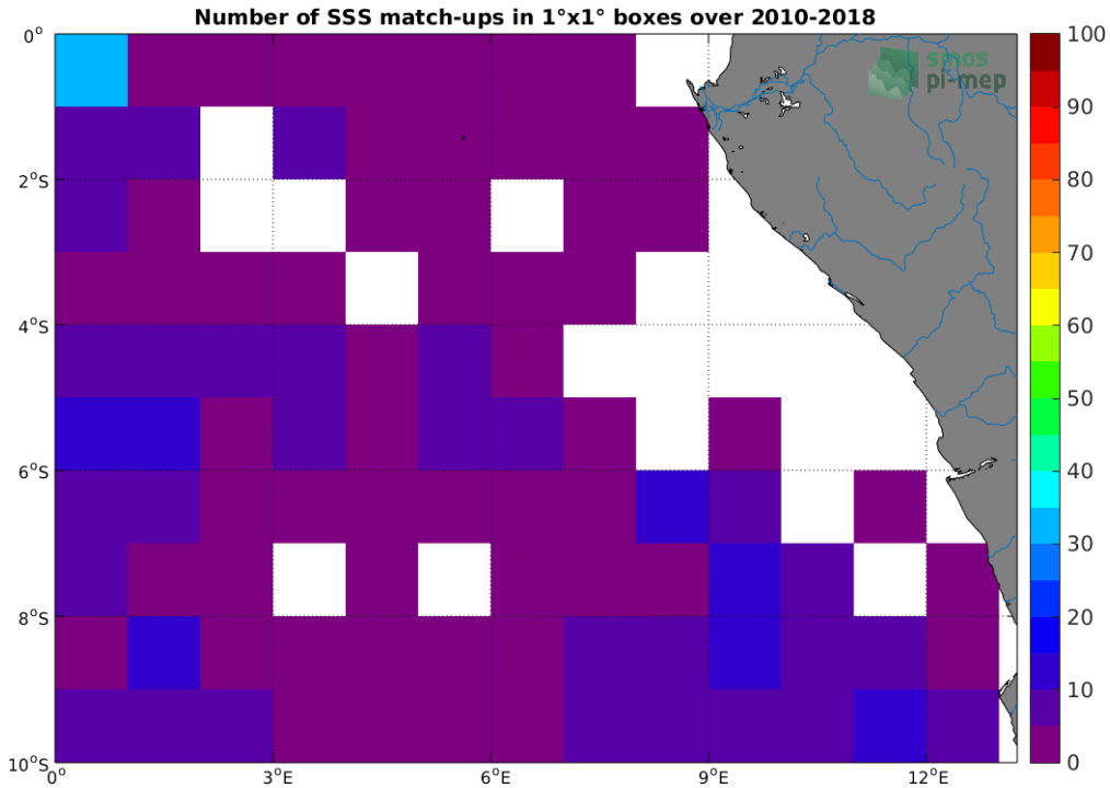
Figure 4: Number of SSS match-ups between Argo SSS and the SMOS-L2-DPGS-v662 SSS product for the Congo river plume Pi-MEP region over 1^\circ \times 1^\circ boxes and for the full satellite product period.
