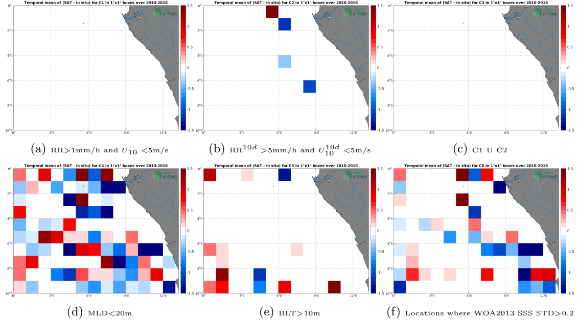
Figure 12: Temporal mean gridded over spatial boxes of size 1^\circ \times 1^\circ of \Delta\text{SSS} (SMOS-L2-DPGS-v662 - Argo) for 6 different subdatasets corresponding to: \text{RR} > 1\text{mm/h} and U_{10} < 5\text{m/s} (a), \text{RR}^{10d} > 5\text{mm/h} and U_{10}^{10d} < 5\text{m/s} (b), C1 U C2 (c), \text{MLD} < 20\text{m} (d), \text{BLT} > 10\text{m} (e), Locations where WOA2013 SSS STD > 0.2 (f).
