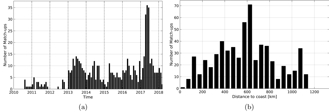
Figure 1: Number of match-ups between Argo and SMOS-L2-DPGS-v662 SSS as a function of time (a) and as function of the distance to coast (b) over the Congo river plume Pi-MEP region and for the full satellite product period.
