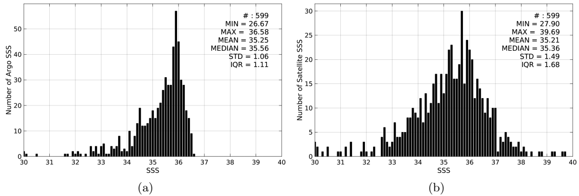
Figure 2: Histograms of SSS from Argo (a) and SMOS-L2-DPGS-v662 (b) considering all match-up pairs per bins of 0.1 over the Congo river plume Pi-MEP region and for the full satellite product period.
