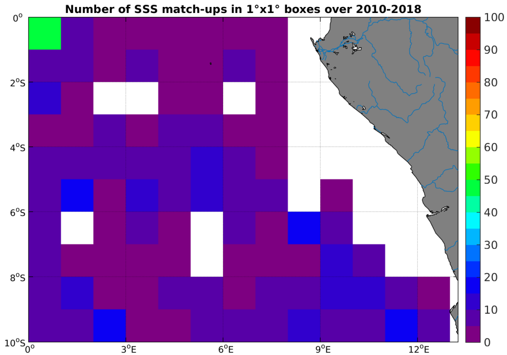
Figure 4: Number of SSS match-ups between Argos SSS and the SMOS-L2-DPGS-v662 SSS product for the Congo river plume Pi-MEP region over 1°x1° boxes and for the full satellite product period.
