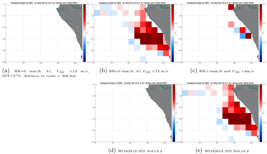
Figure 12: Temporal mean gridded over spatial boxes of size 1^\circ \times 1^\circ of \Delta SSS (SMAP SSS L4 OI v1 - 7day (IPRC) - TSG (LEGOS-DM)) for 5 different subdatasets corresponding to:RR=0 mm/h, 3 < U_{10} < 12 m/s, SST>5°C, distance to coast > 800 km (a), RR=0 mm/h, 3 < U_{10} < 12 m/s (b), RR>1mm/h and U_{10} < 4 m/s (c), WOA2013 SSS Std<0.2 (d), WOA2013 SSS Std>0.2 (e).
