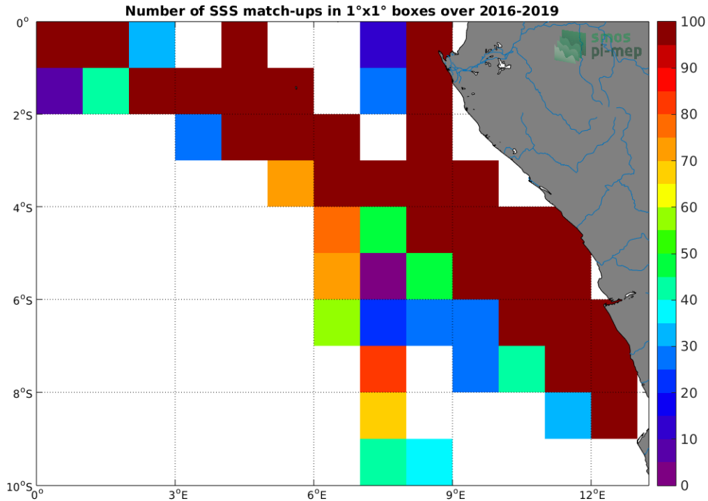
Figure 4: Number of SSS match-ups between TSG (LEGOS-DM) SSS and the SMAP SSS L4 OI v1 - 7day (IPRC) SSS product for the Congo river plume Pi-MEP region over 1^\circ \times 1^\circ boxes and for the full satellite product period.
