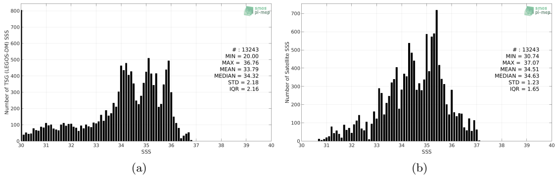
Figure 2: Histograms of SSS from TSG (LEGOS-DM) (a) and SMAP SSS L4 OI v1 - 7day (IPRC) (b) considering all match-up pairs per bins of 0.1 over the Congo river plume Pi-MEP region and for the full satellite product period.
