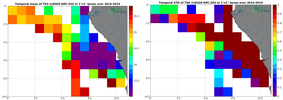
(c) MEAN(TSG (LEGOS-DM) SSS)
