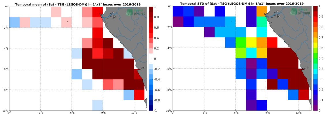
(e) MEAN( \Delta SSS) (Satellite - TSG (LEGOS-DM))
