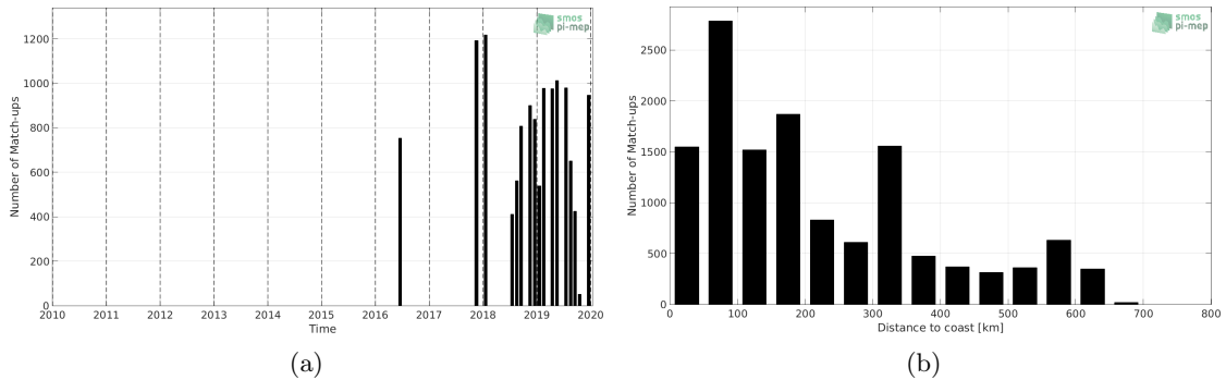
Figure 1: Number of match-ups between TSG (LEGOS-DM) and SMAP SSS L4 OI v1 - 7day (IPRC) SSS as a function of time (a) and as function of the distance to coast (b) over the Congo river plume Pi-MEP region and for the full satellite product period.
