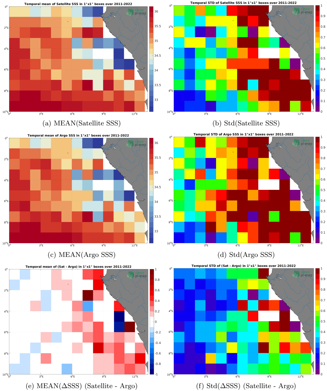
Figure 6: Temporal mean (left) and Std (right) of SSS from SMAP SSS L4 OI v1 - 7 Days (IPRC) (top), Argo (middle), and of \Delta SSS (Satellite - Argo). Only match-up pairs are used to generate these maps.
